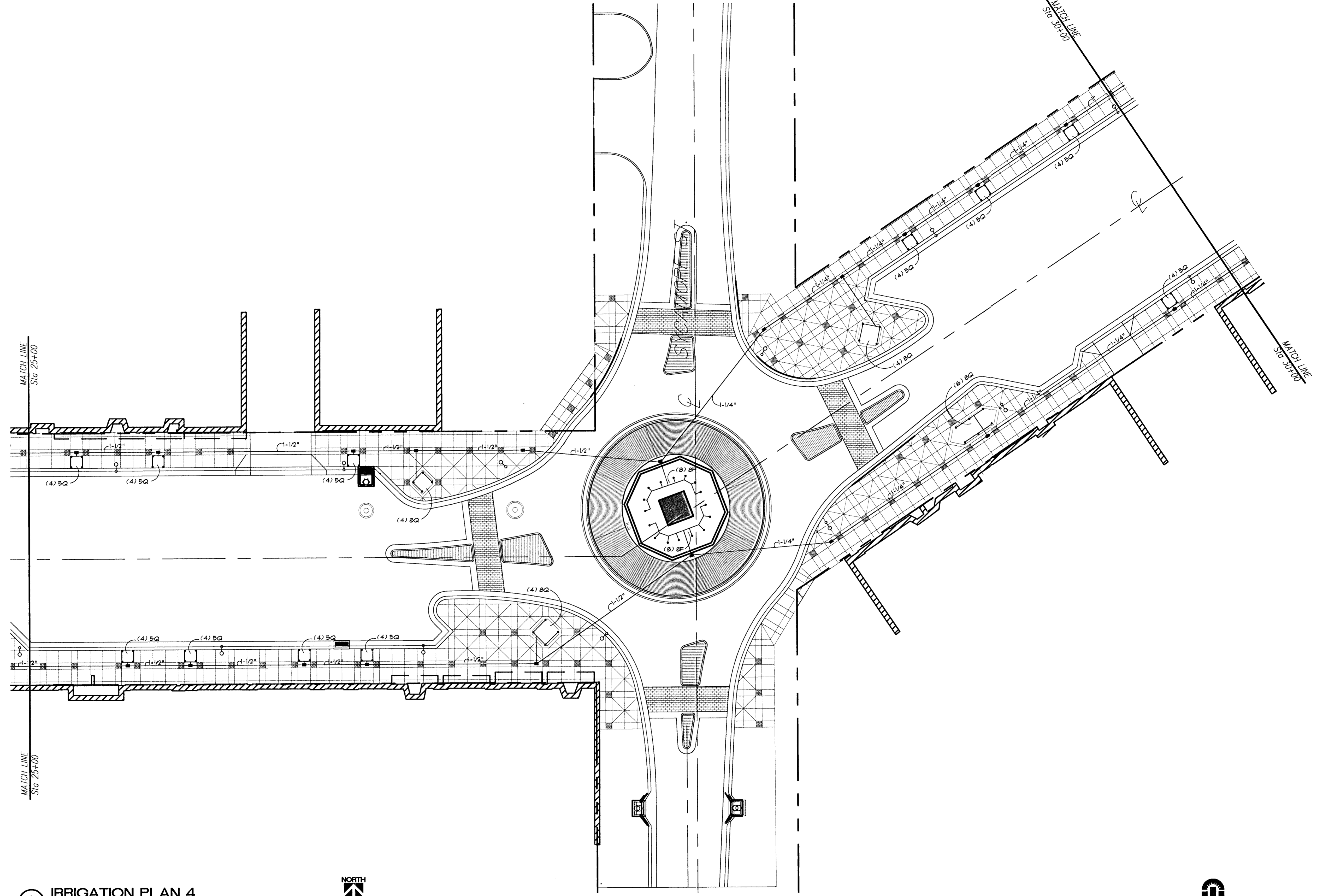
(A) IRRIGATION PLAN 4
