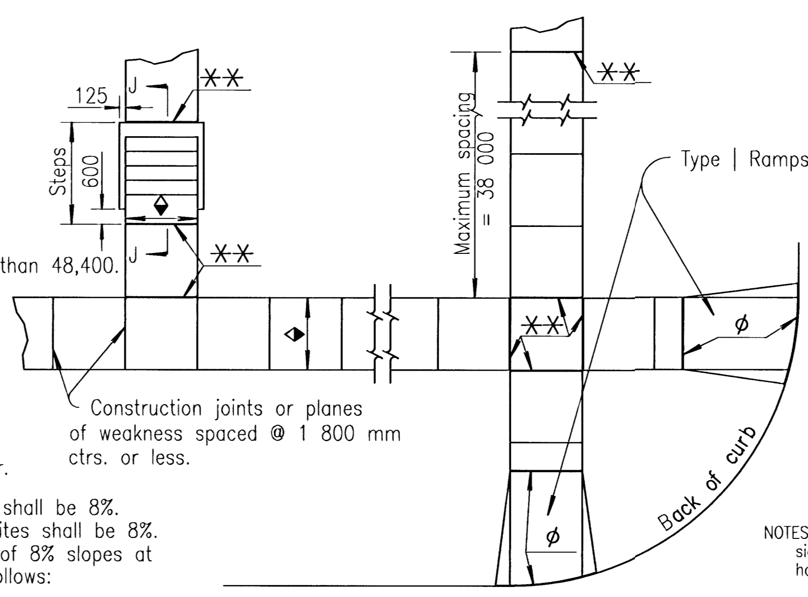
TYPICAL PLAN
