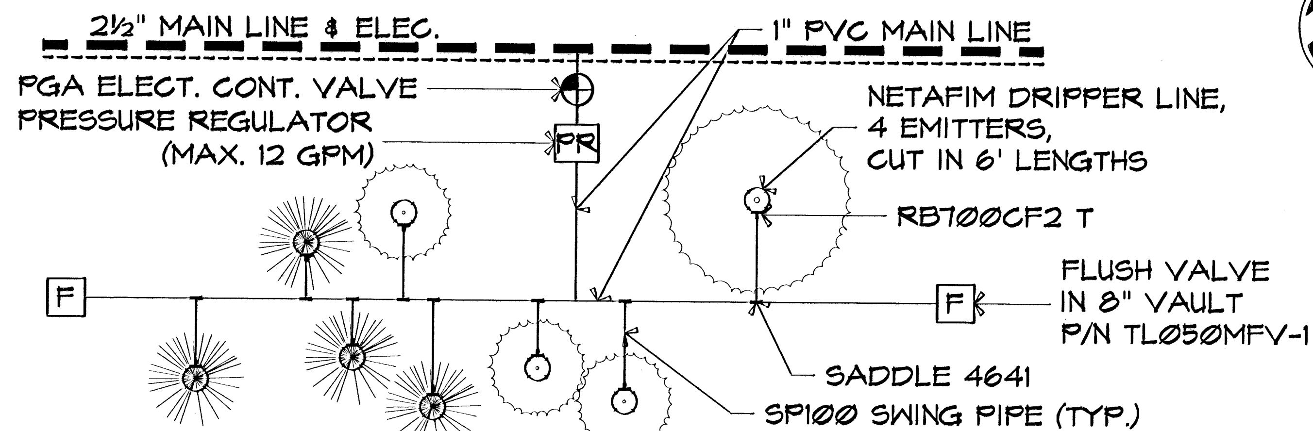
DRIP IRRIGATION DETAIL (TYP.) NO SCALE
