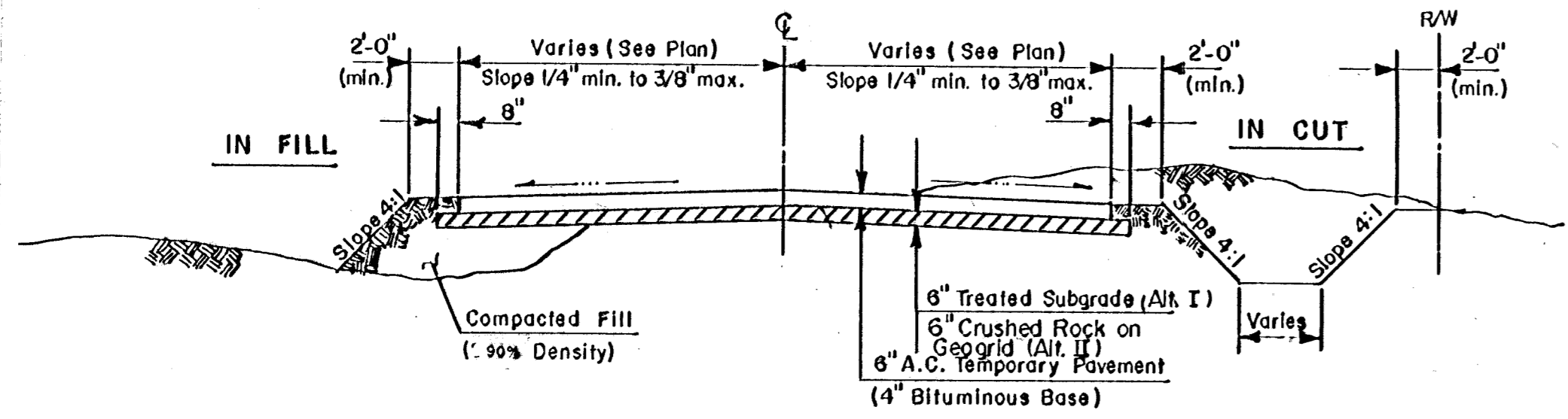
TYPICAL SECTION TEMPORARY A.C. PAVEMENT
