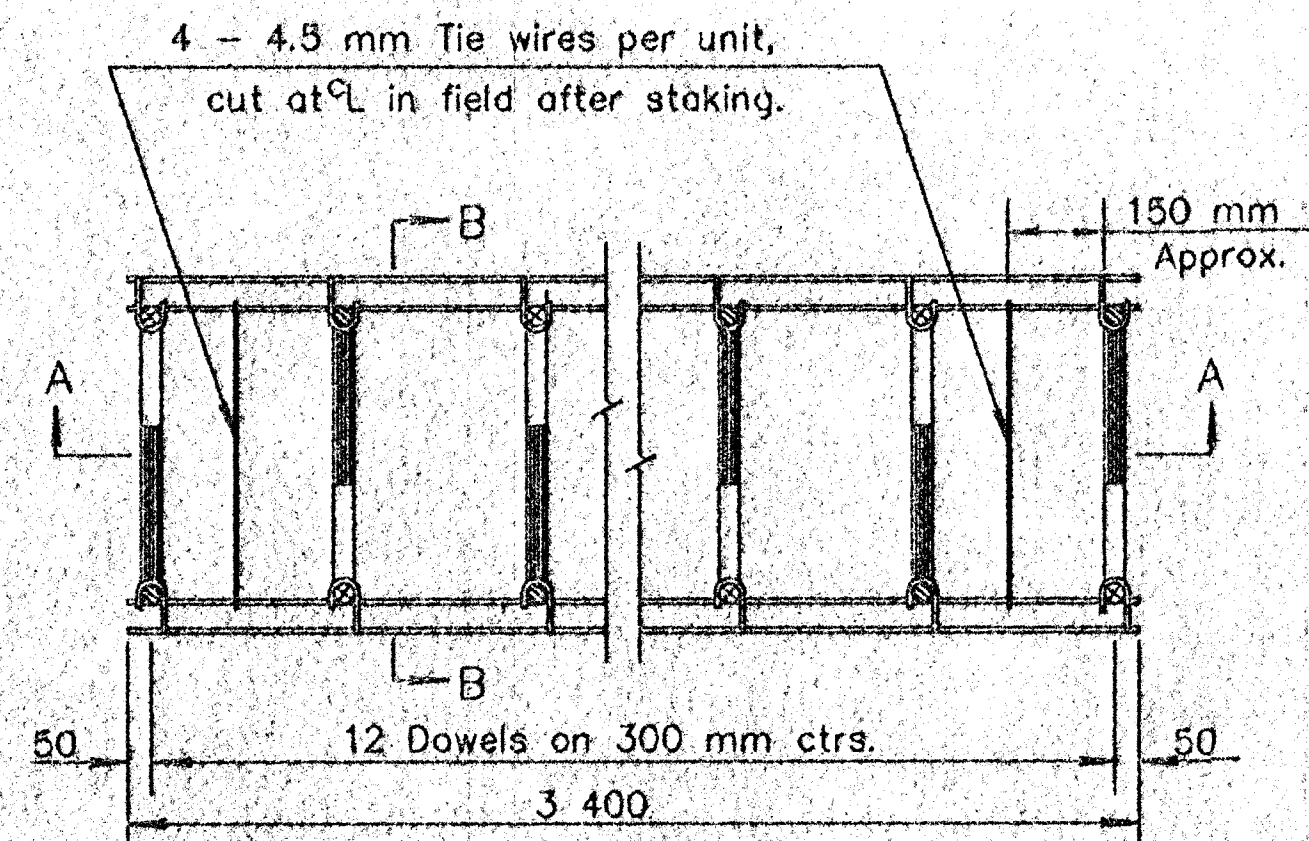
PLAN VIEW
