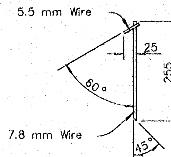
STAKE DETAIL
