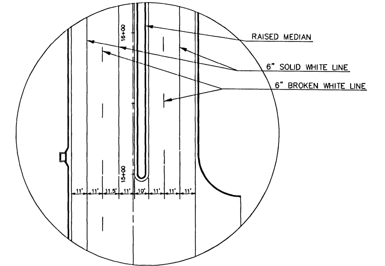
DETAIL FOR STA. 15+00 THRU 17+50
