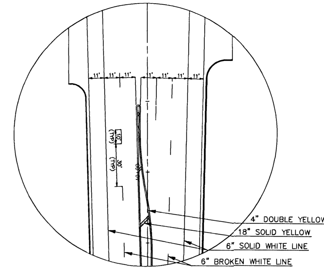
DETAIL FOR STA. 7+00 THRU 15+00
