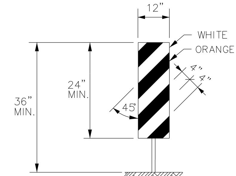
VERTICAL PANEL
