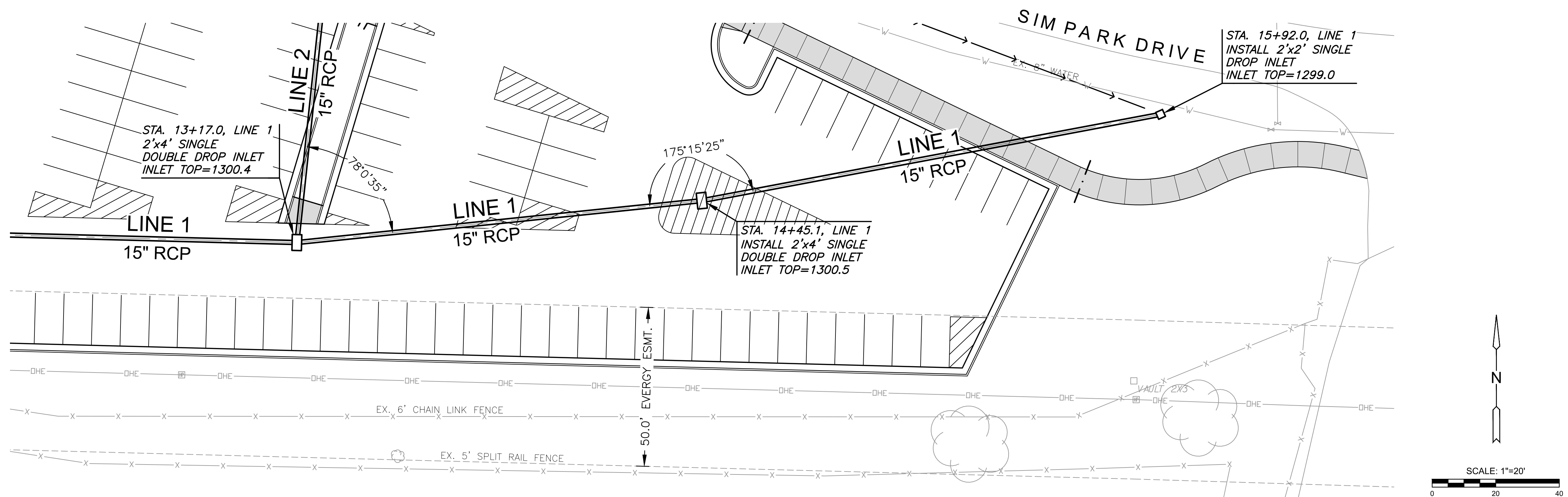
PLAN LINE 1 CONT. PROFILE LINE 1 CONT.
