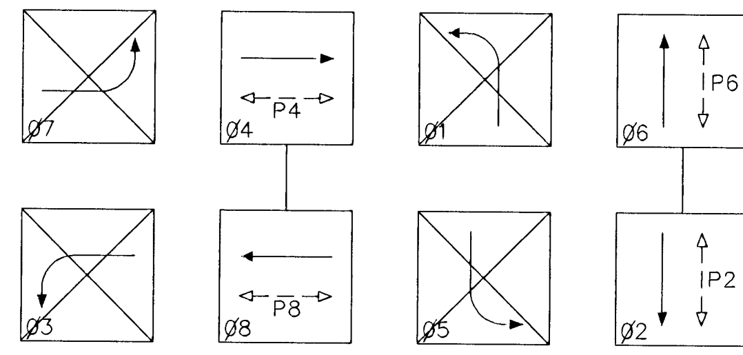
Signal Phasing
