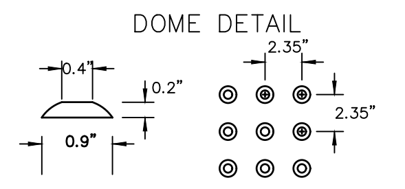
DOME DETAIL
