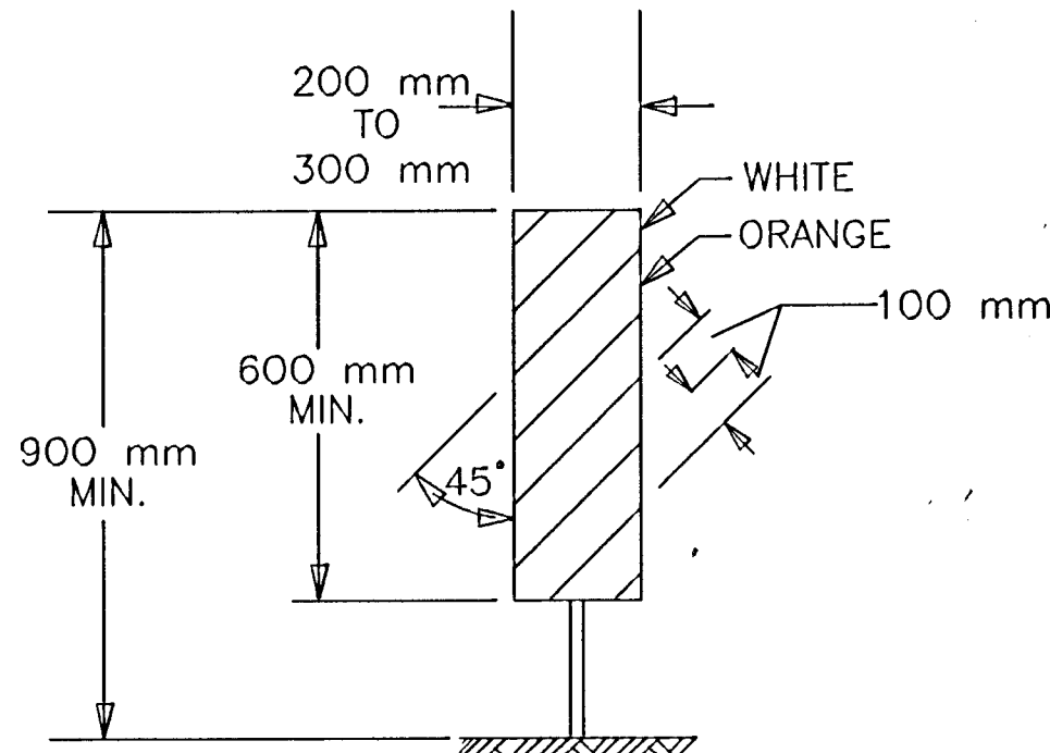
VERTICAL PANEL
