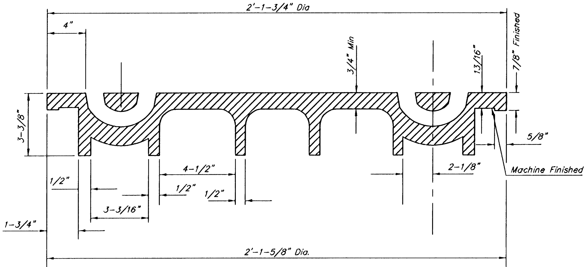
SECTION VIEW
