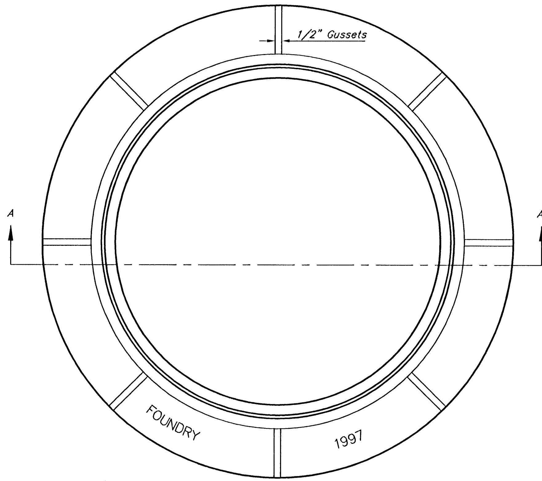
TOP VIEW
