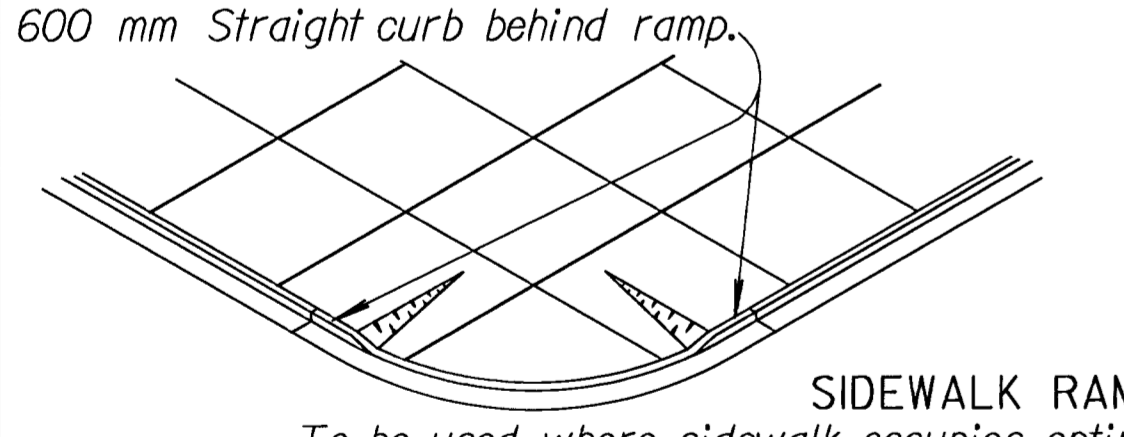
PLAN VIEW
