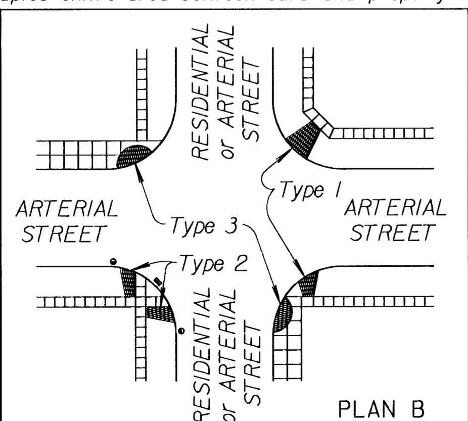
SIDEWALK RAMP TYPE 3 To be used where sidewalk occupies entire area between curb and property line.
