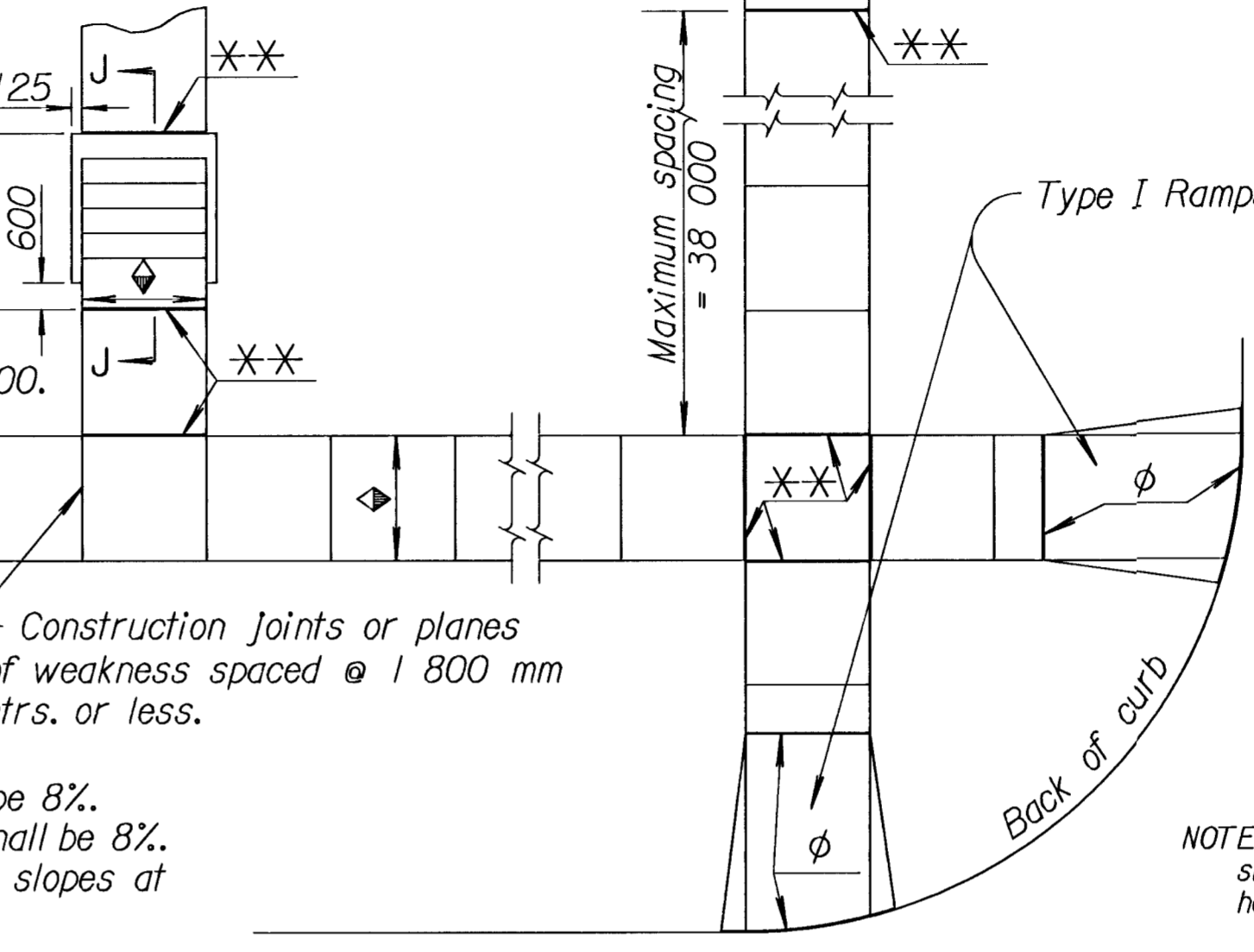
TYPICAL PLAN
