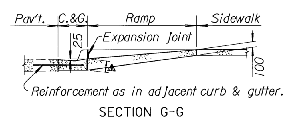
SECTION G-G
