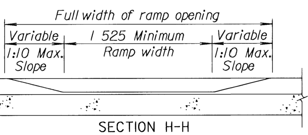
SIDEWALK RAMP TYPE 3 To be used where sidewalk occupies entire area between curb and property line.
