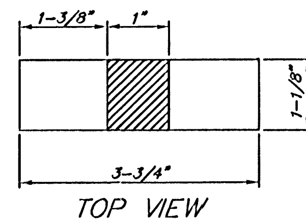
PICKHOLE DETAIL
