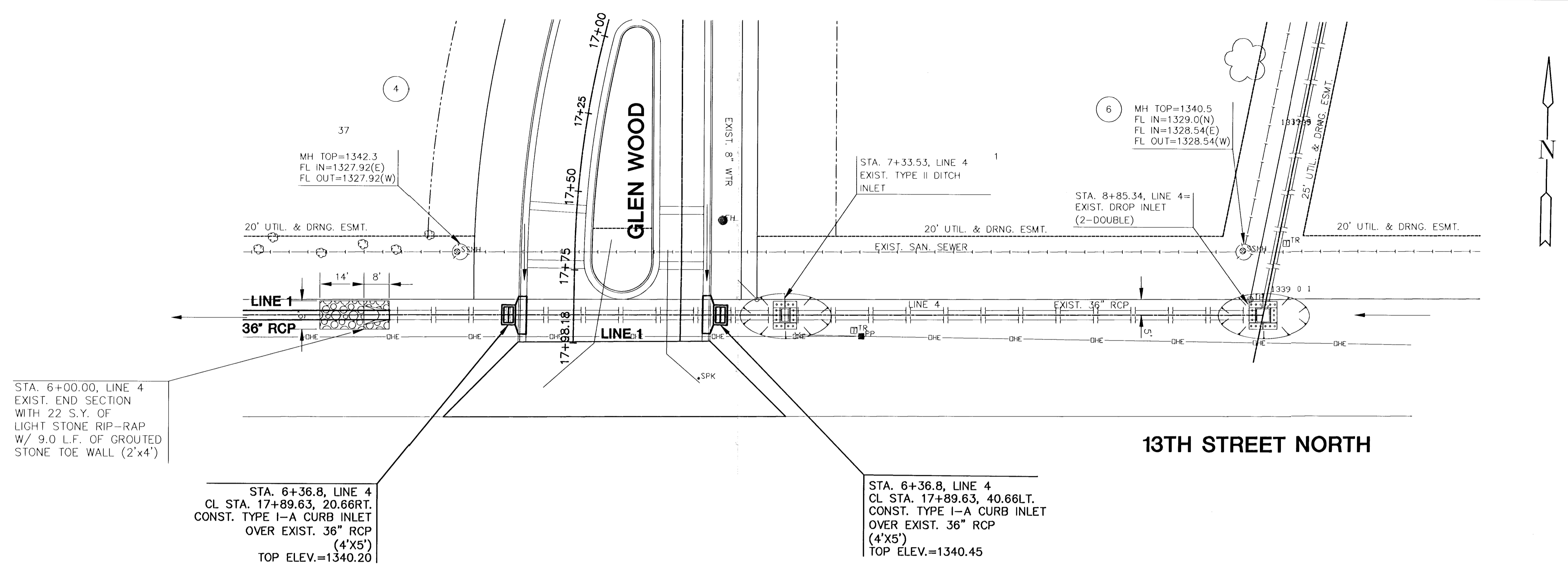
PLAN LINE 1 SCALE: 1"=20'
