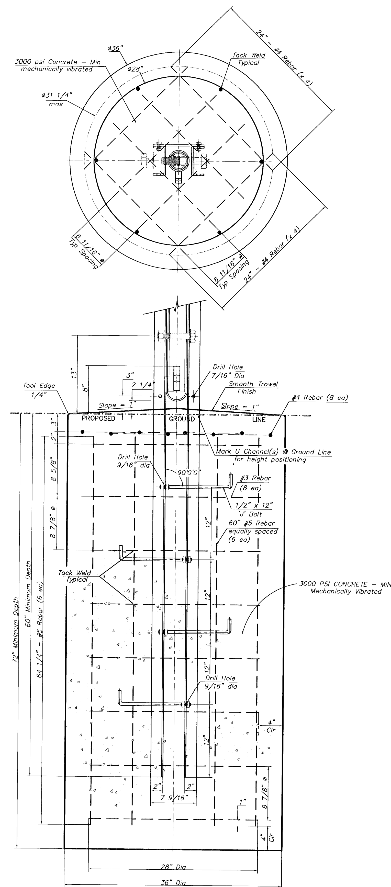
SECTION B-B
