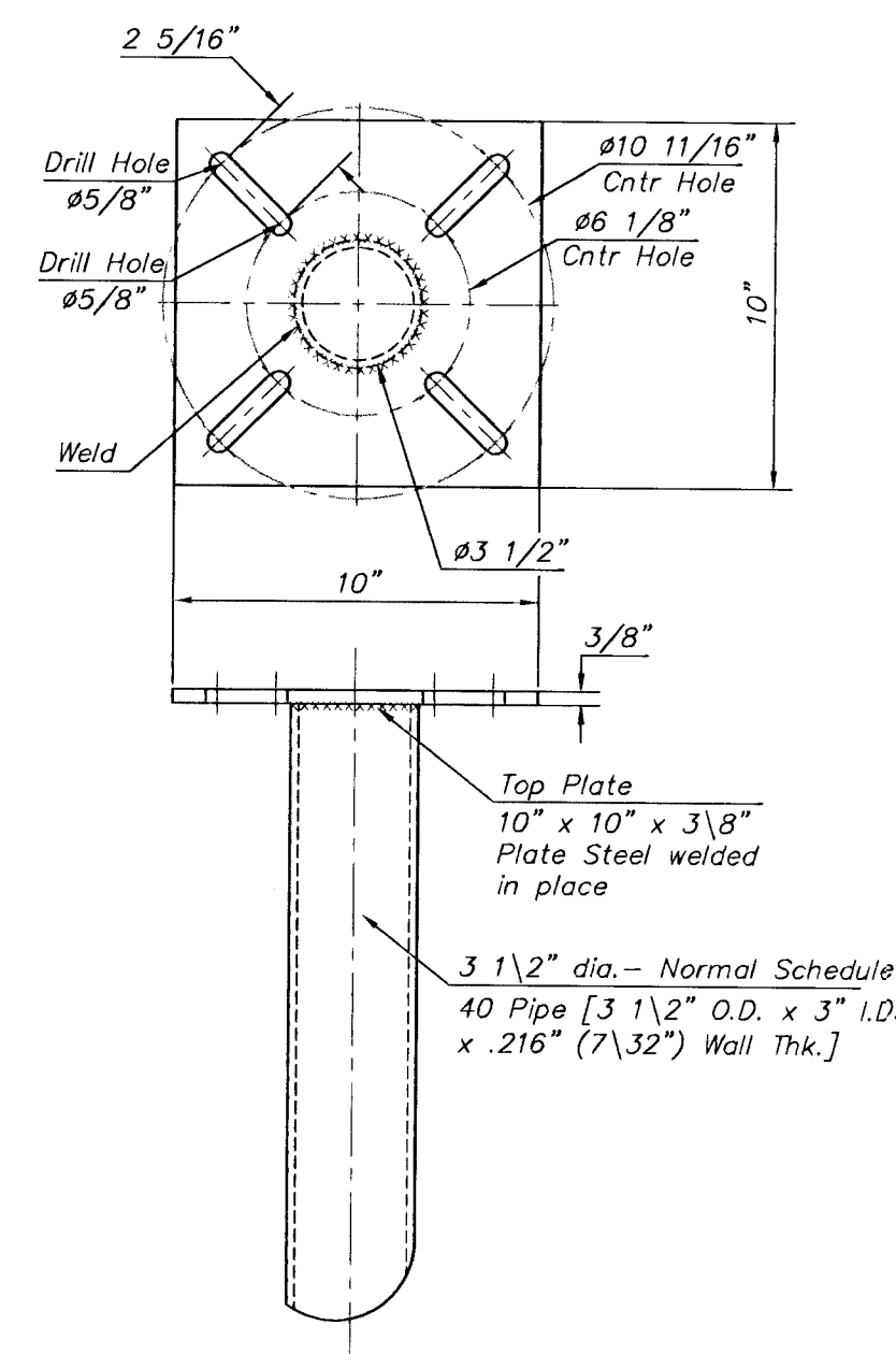
POLE TOP DETAIL
