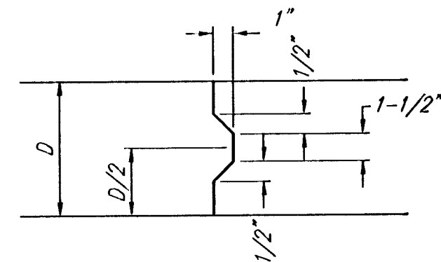
KEYWAY DETAIL
