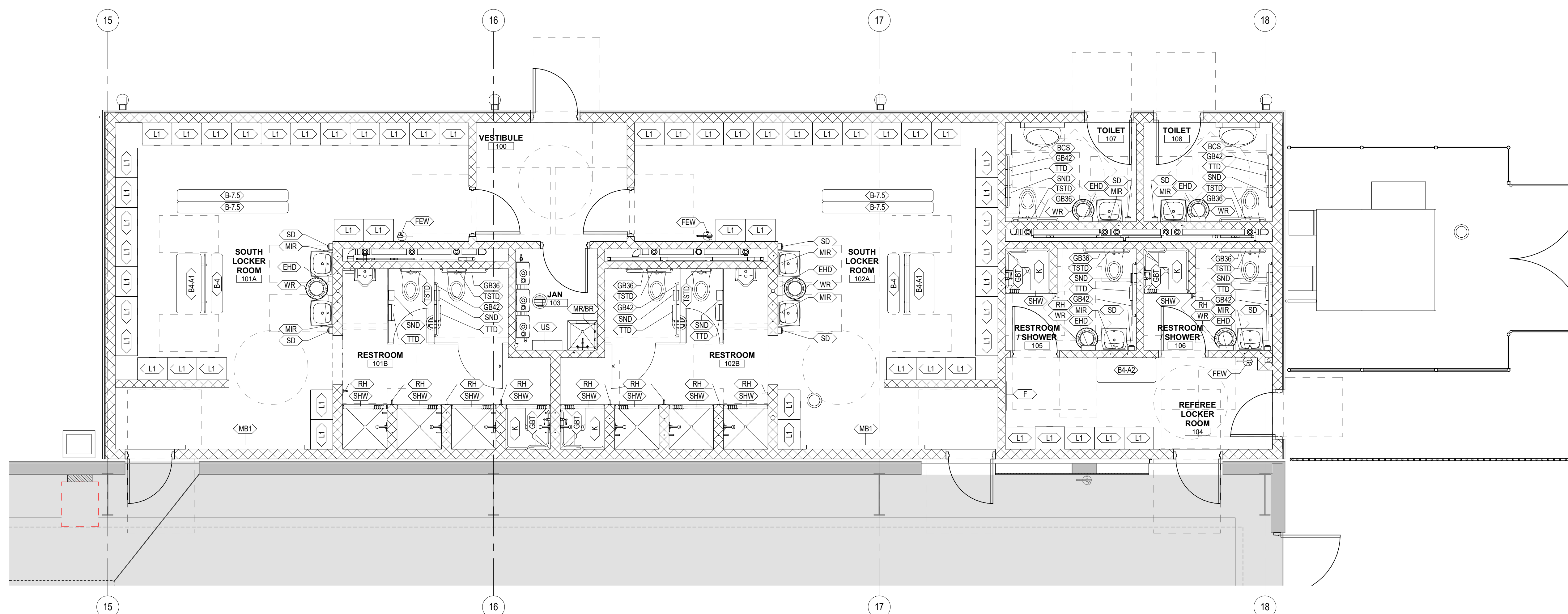
B SOUTH LOCKER ROOM EQUIPMENT PLAN 1/4" = 1'-0"
