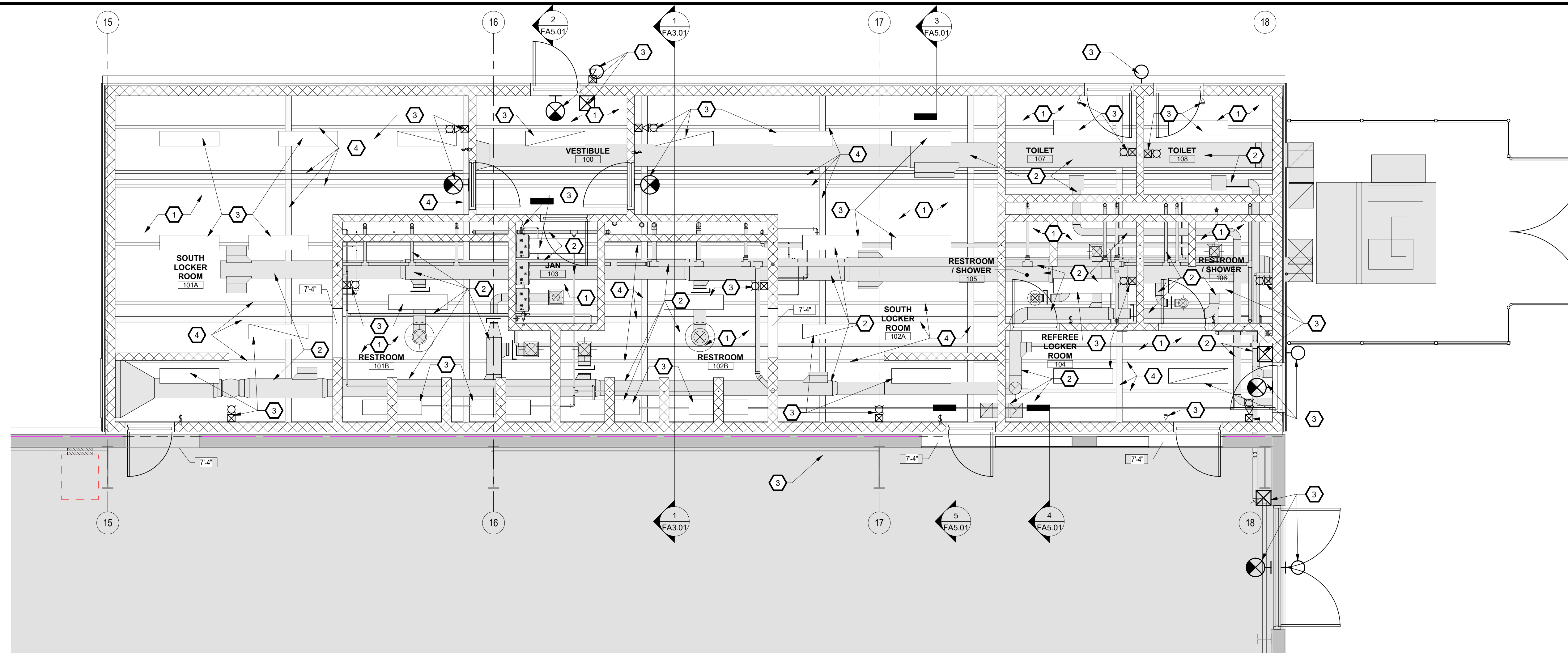
A SOUTH LOCKER - REFLECTED CEILING PLAN 1/4" = 1'-0"
