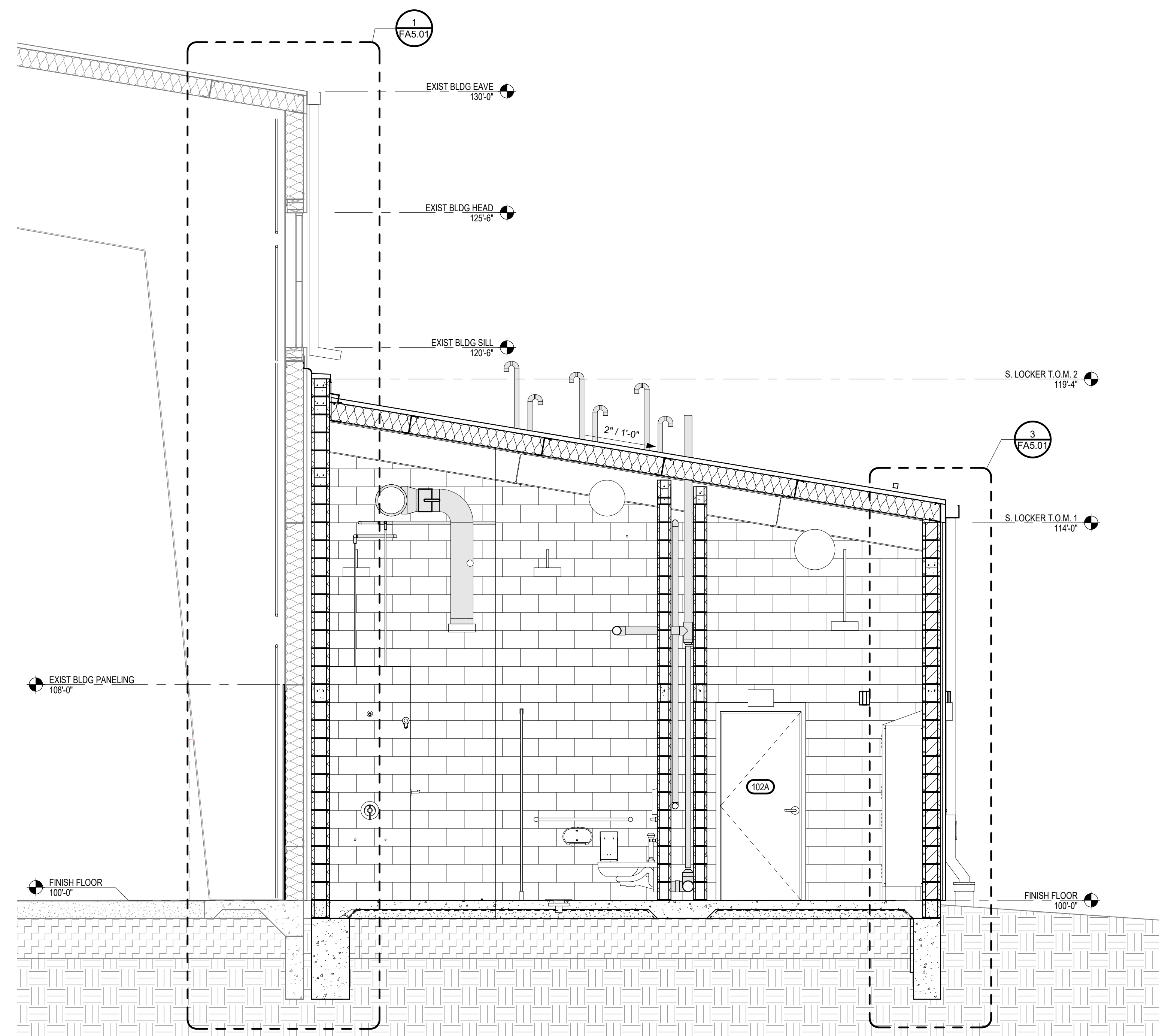
1 BUILDING SECTION - SOUTH LOCKER 3/8" = 1'-0"
