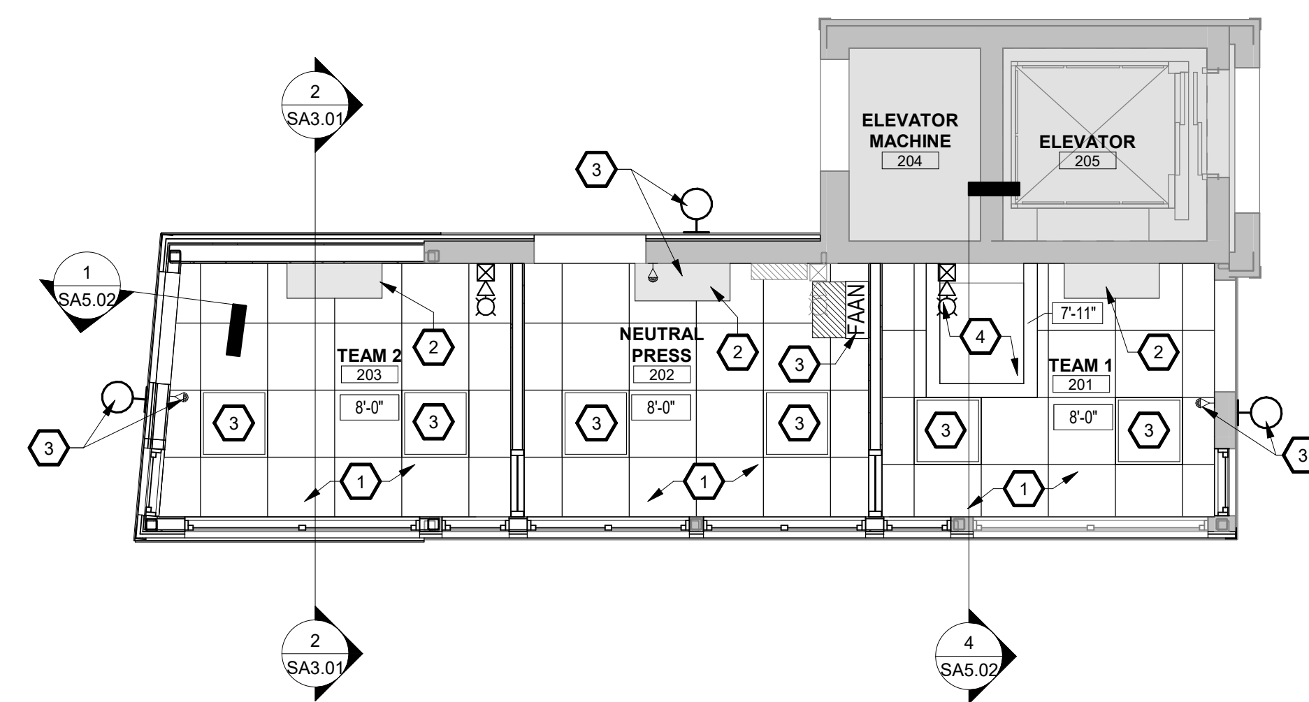
A PRESSBOX - REFLECTED CEILING PLAN 1/4" = 1'-0" 0 2 4 6 8 NORTH
