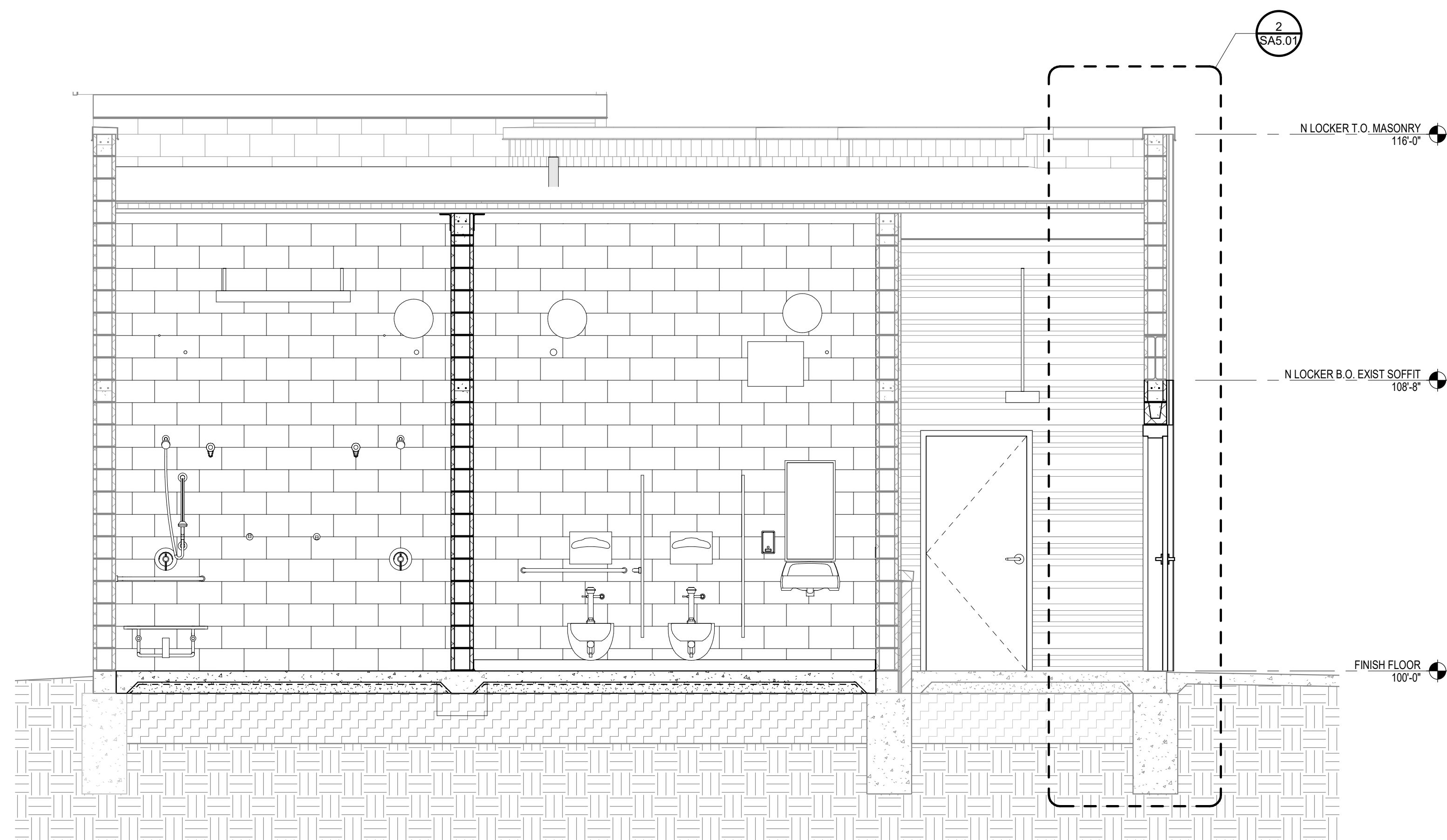
3 BUILDING SECTION - NORTH LOCKER 3/8" = 1'-0"
