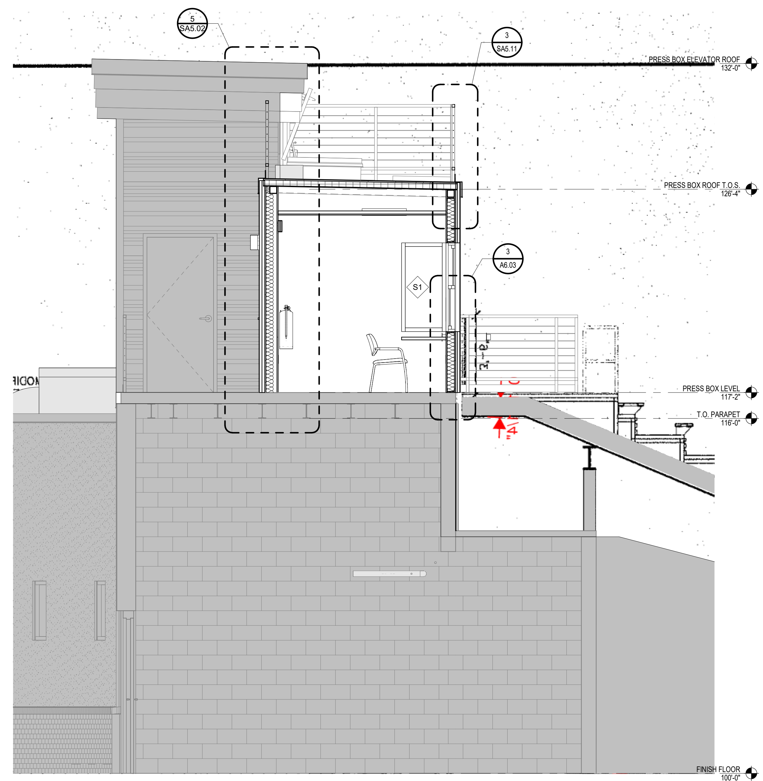
2 BUILDING SECTION - PRESSBOX 3/8" = 1'-0"
