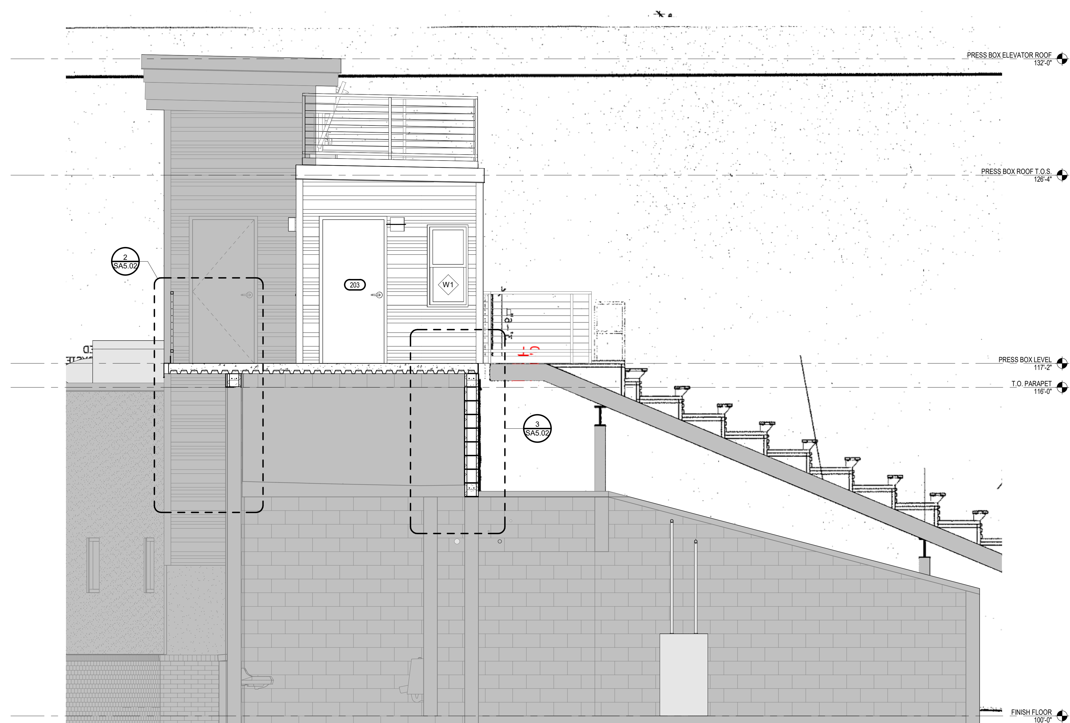
1 BUILDING SECTION - PRESSBOX 3/8" = 1'-0"
