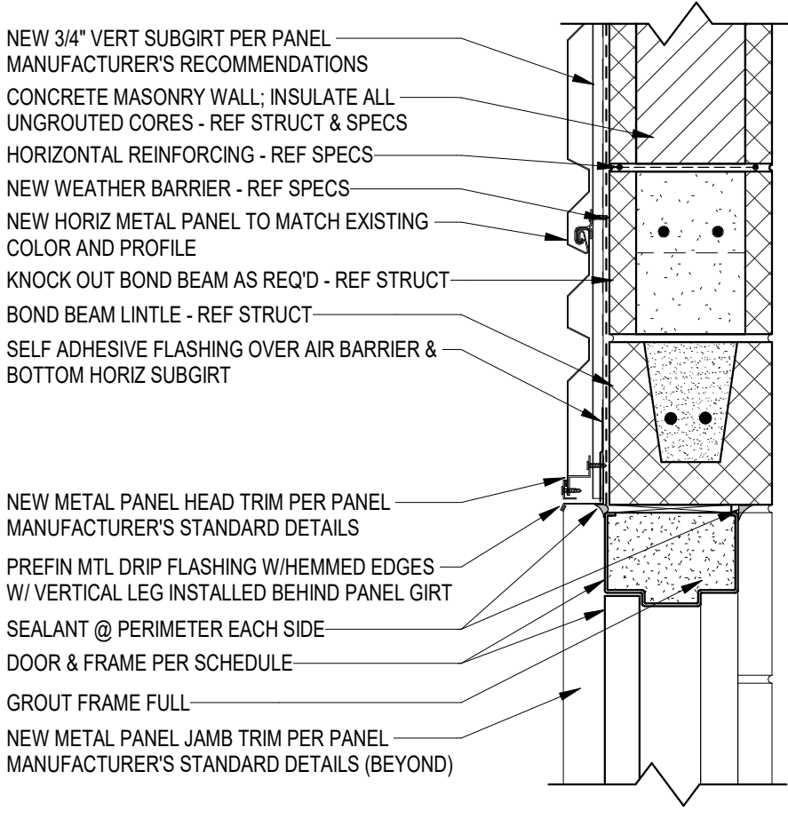
12 DOOR HEAD @ CMU & HORIZ MTL PANEL 1 1/2" = 1'-0"
