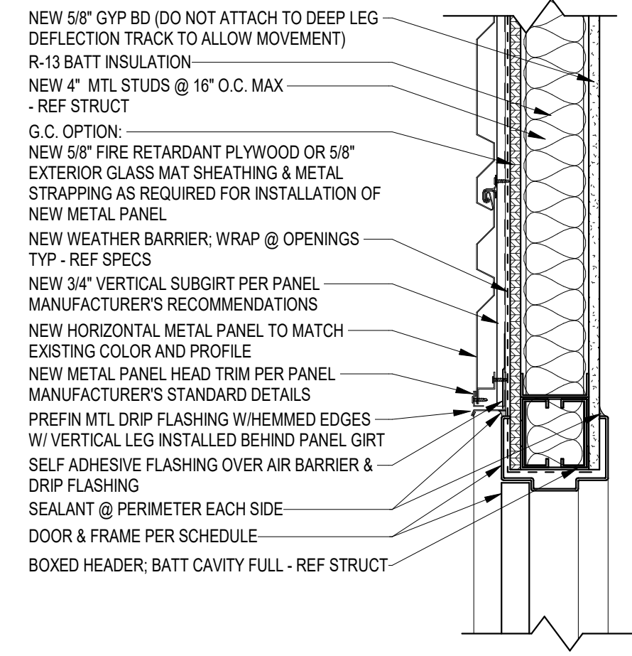
6 DOOR HEAD @ MTL PANEL 1 1/2" = 1'-0"
