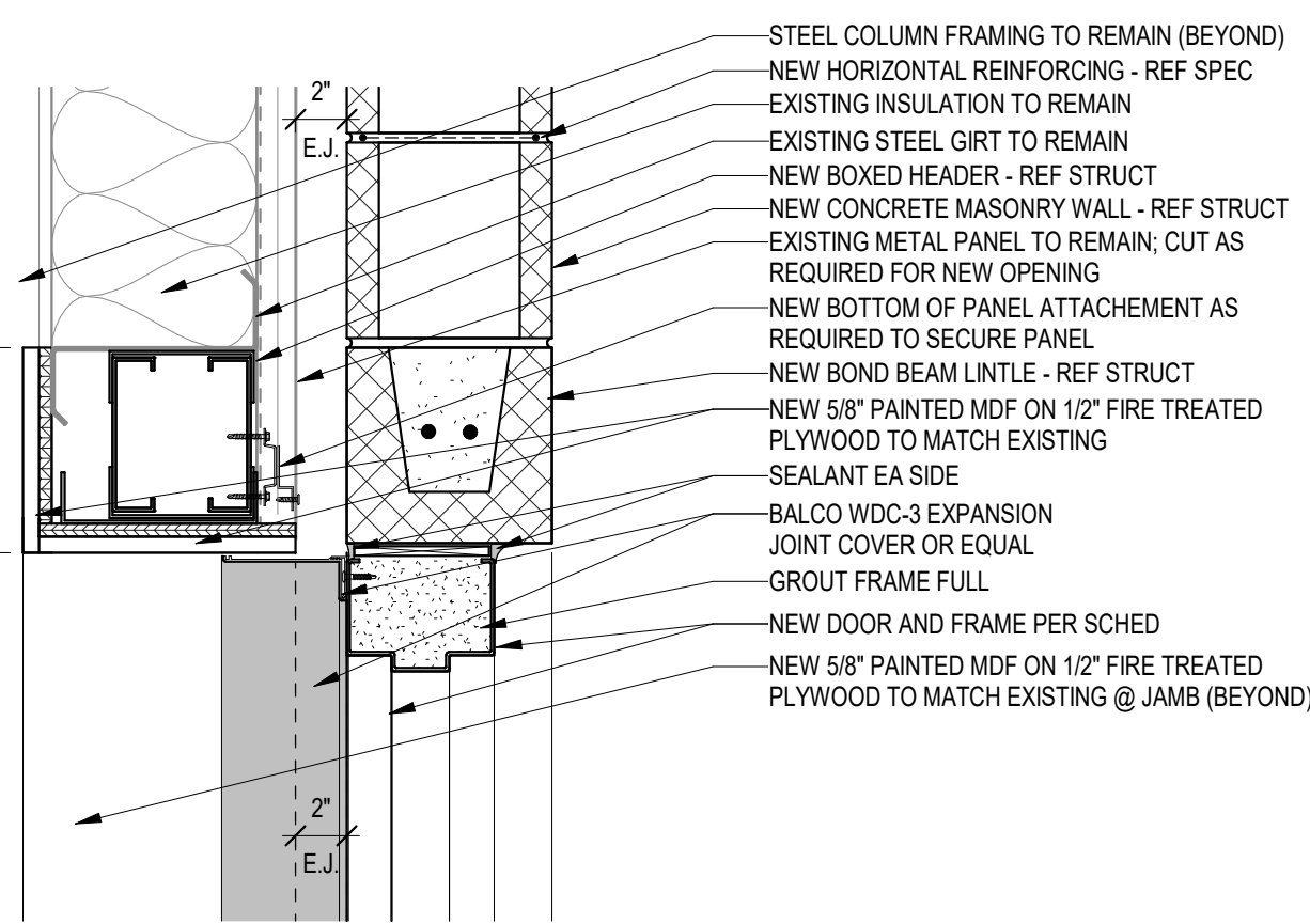
3 HM DOOR HEAD @ EXPANSION JT 1 1/2" = 1'-0"
