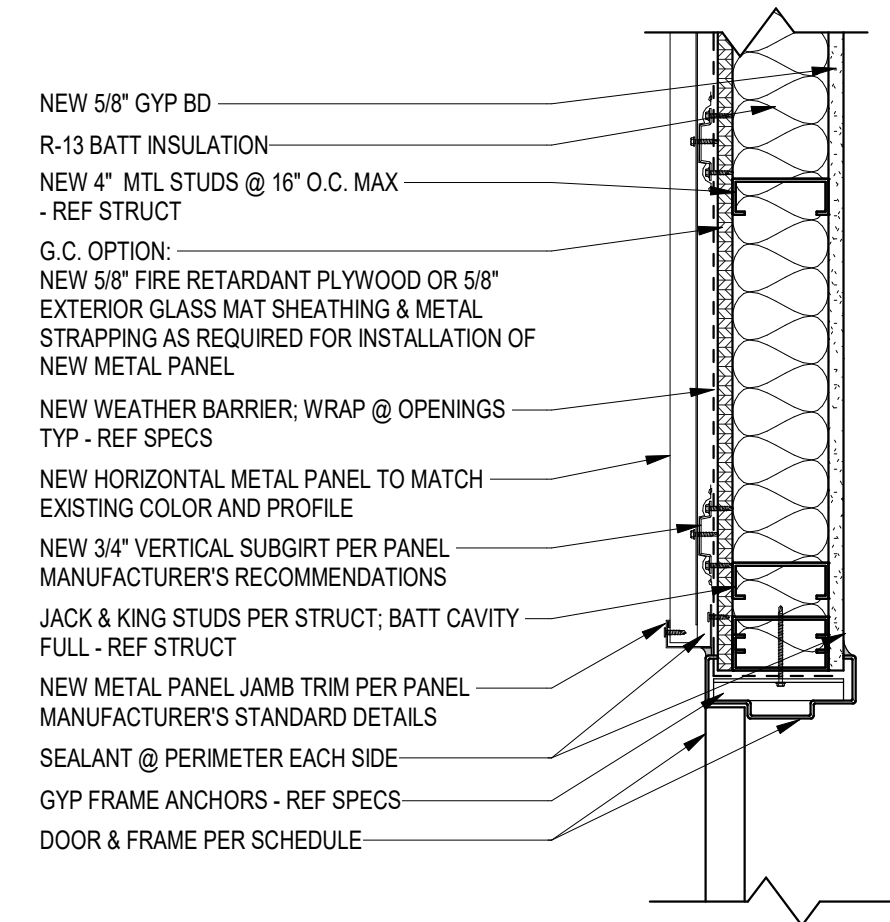
7 DOOR JAMB @ MTL PANEL 1 1/2" = 1'-0"
