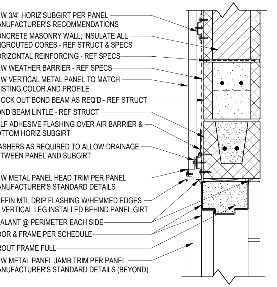
8 DOOR HEAD @ CMU & VERT MTL PANEL 1 1/2" = 1'-0"
