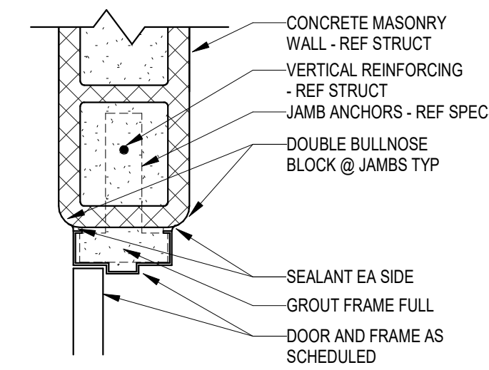
2 HM DOOR JAMB @ CMU 1 1/2" = 1'-0"
