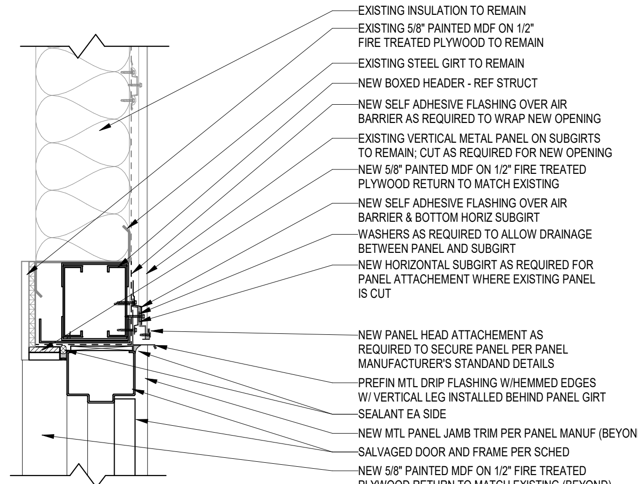
10 HM DOOR HEAD @ EXISTING PANEL 1 1/2" = 1'-0"
