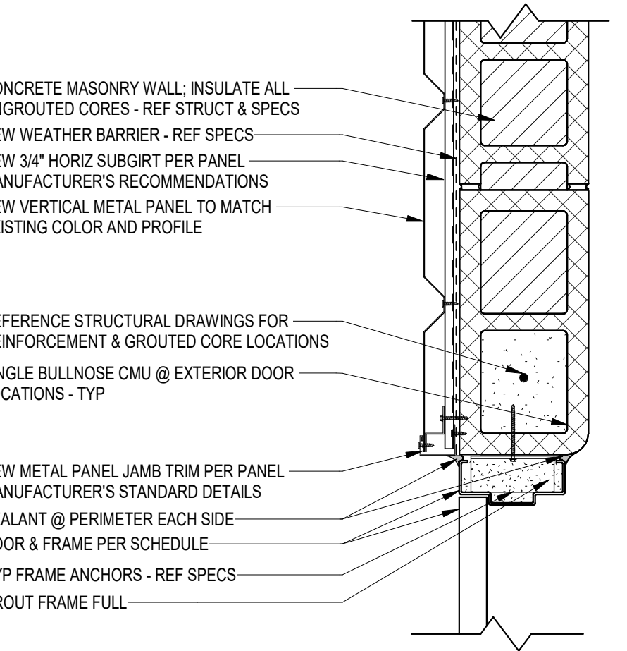
9 DOOR JAMB @ CMU & VERT MTL PANEL 1 1/2" = 1'-0"
