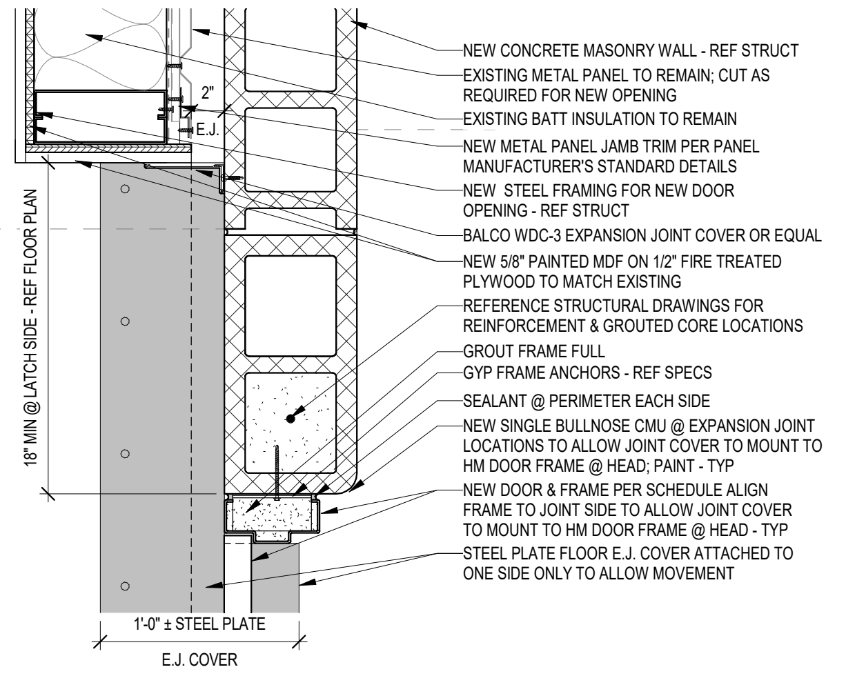
4 HM DOOR JAMB @ EXPANSION JT 1 1/2" = 1'-0"
