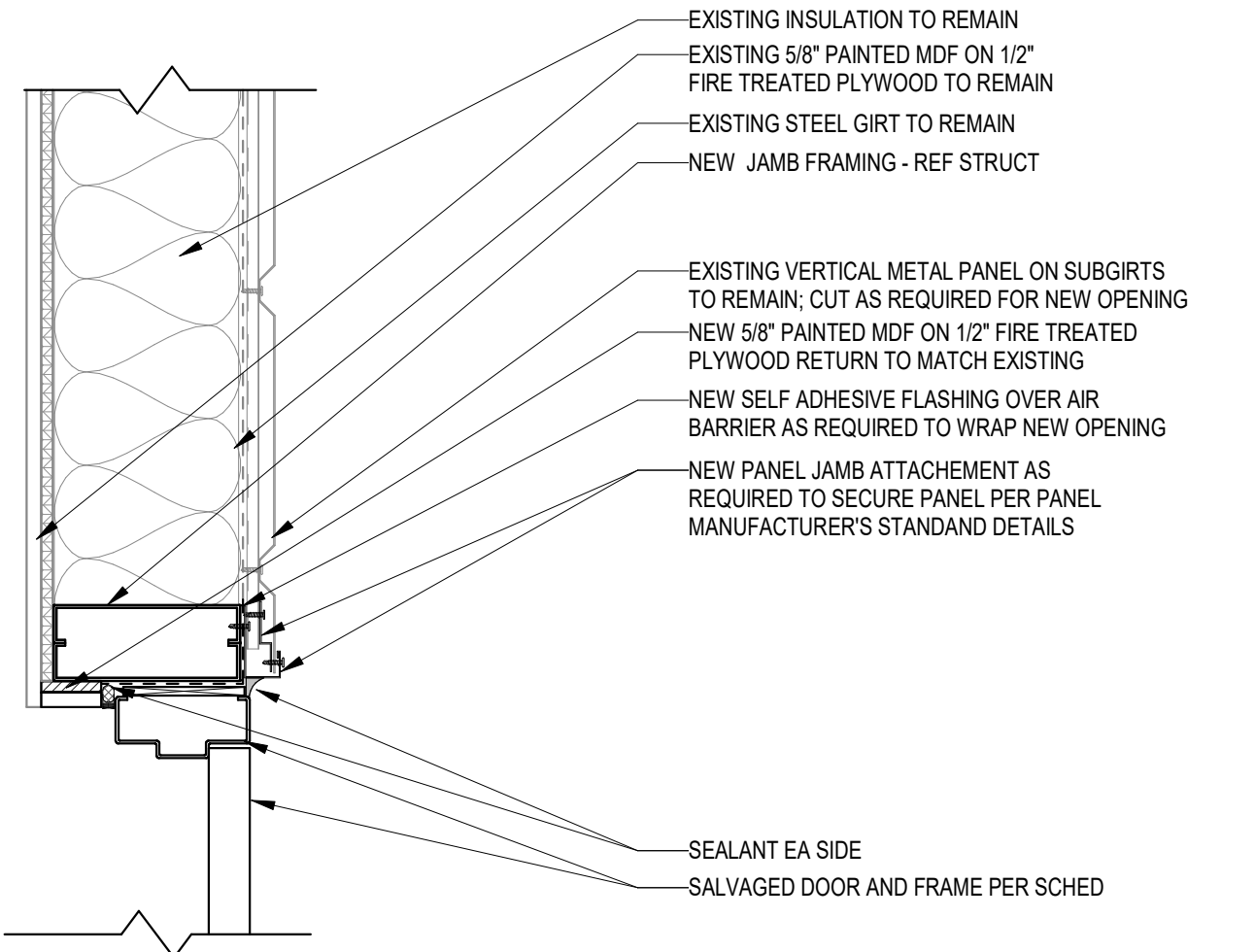
11 HM DOOR JAMB @ EXISTING PANEL 1 1/2" = 1'-0"
