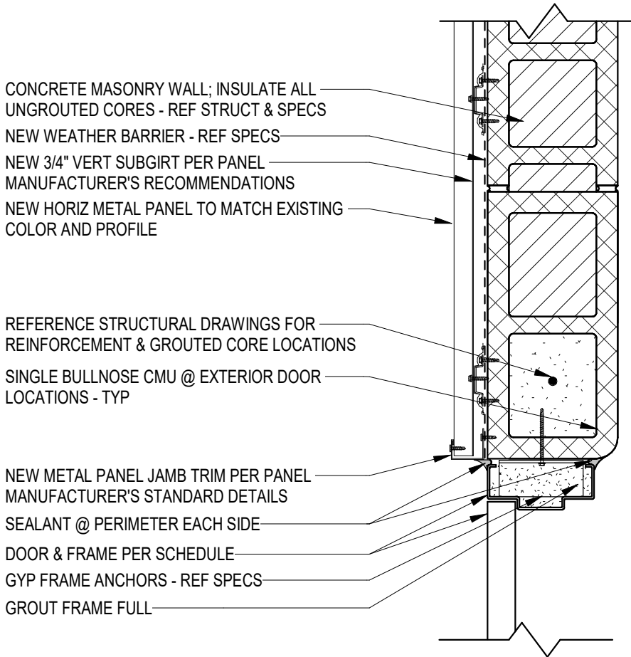
13 DOOR JAMB @ CMU & HORIZ MTL PANEL 1 1/2" = 1'-0"
