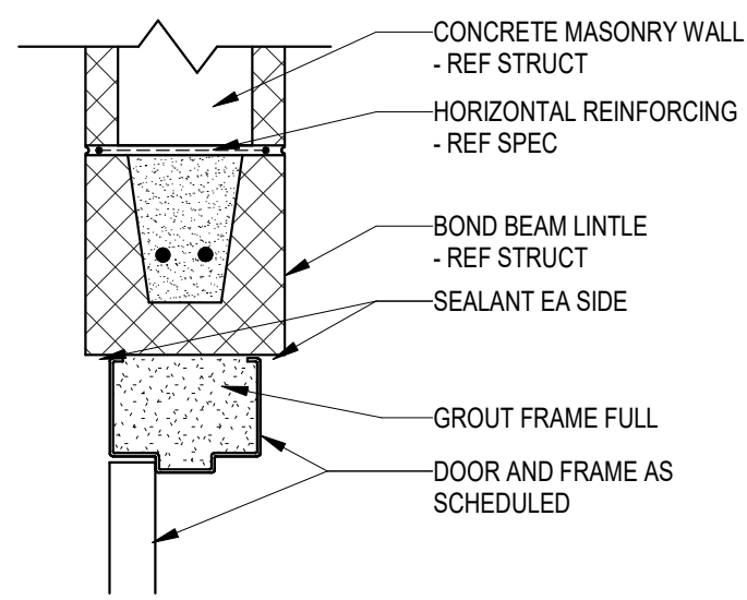
1 HM DOOR HEAD @ CMU 1 1/2" = 1'-0"
