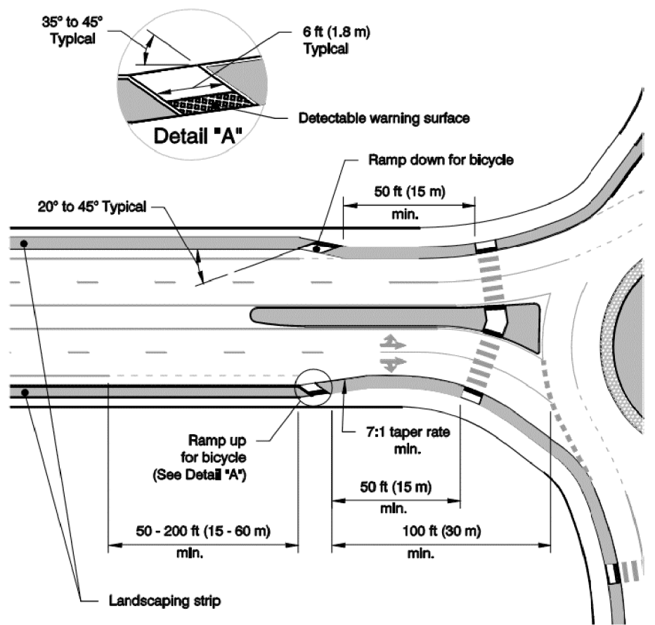
TYPICAL SLIP RAMP DETAIL NCHRP REPORT 672 EXHIBIT 6-67
