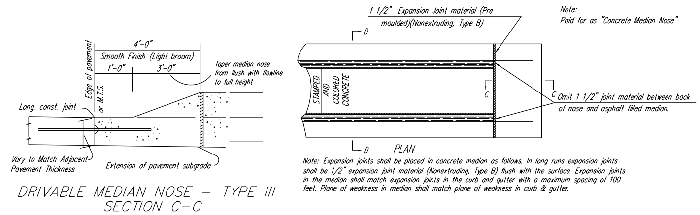
TYPICAL NOSE DETAILS FOR RAISED MEDIANS
