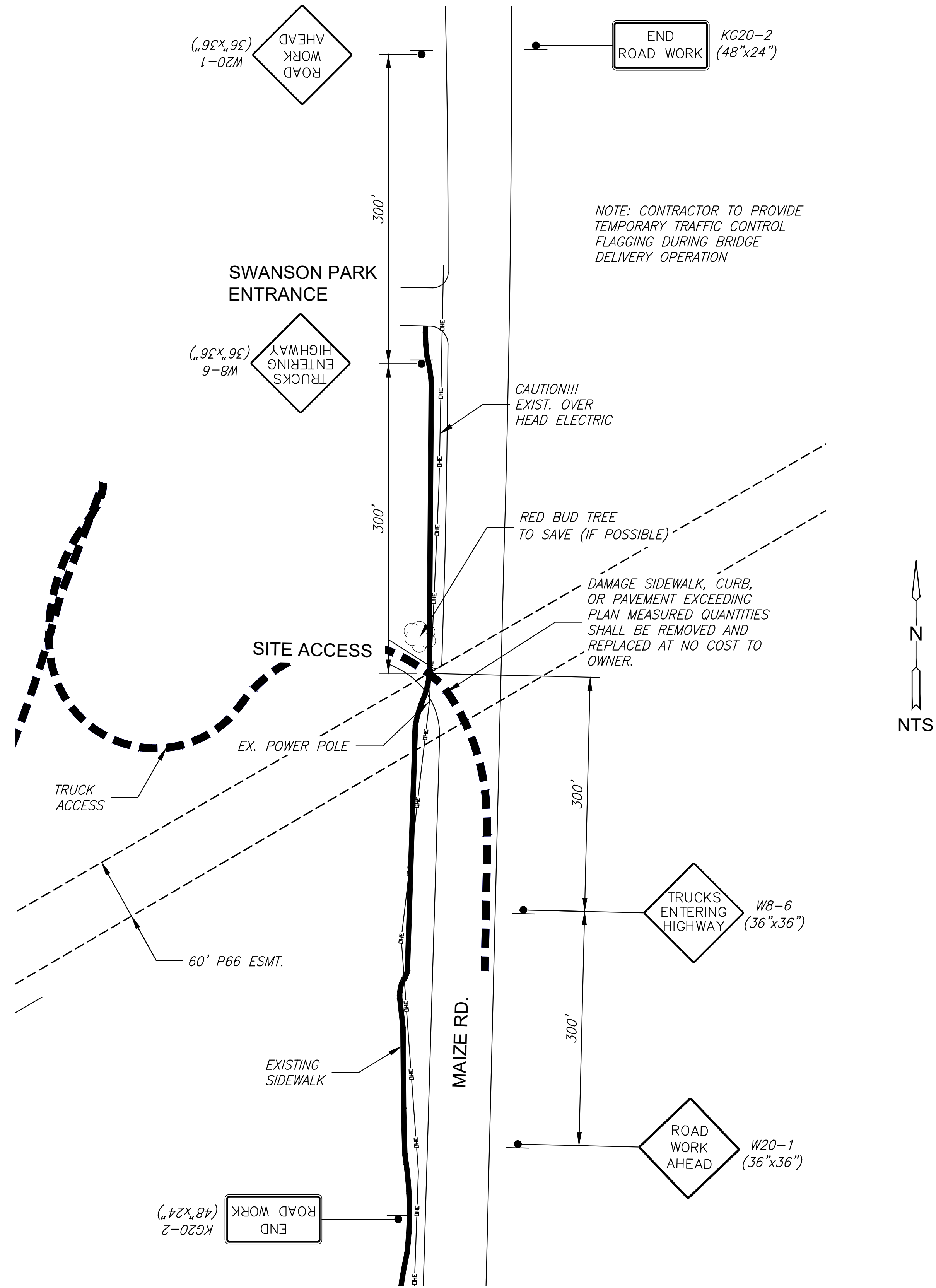
MAIZE RD. TRAFFIC CONTROL PLAN
