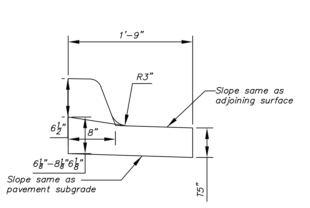
Combined Curb & Gutter (1 1/2")
