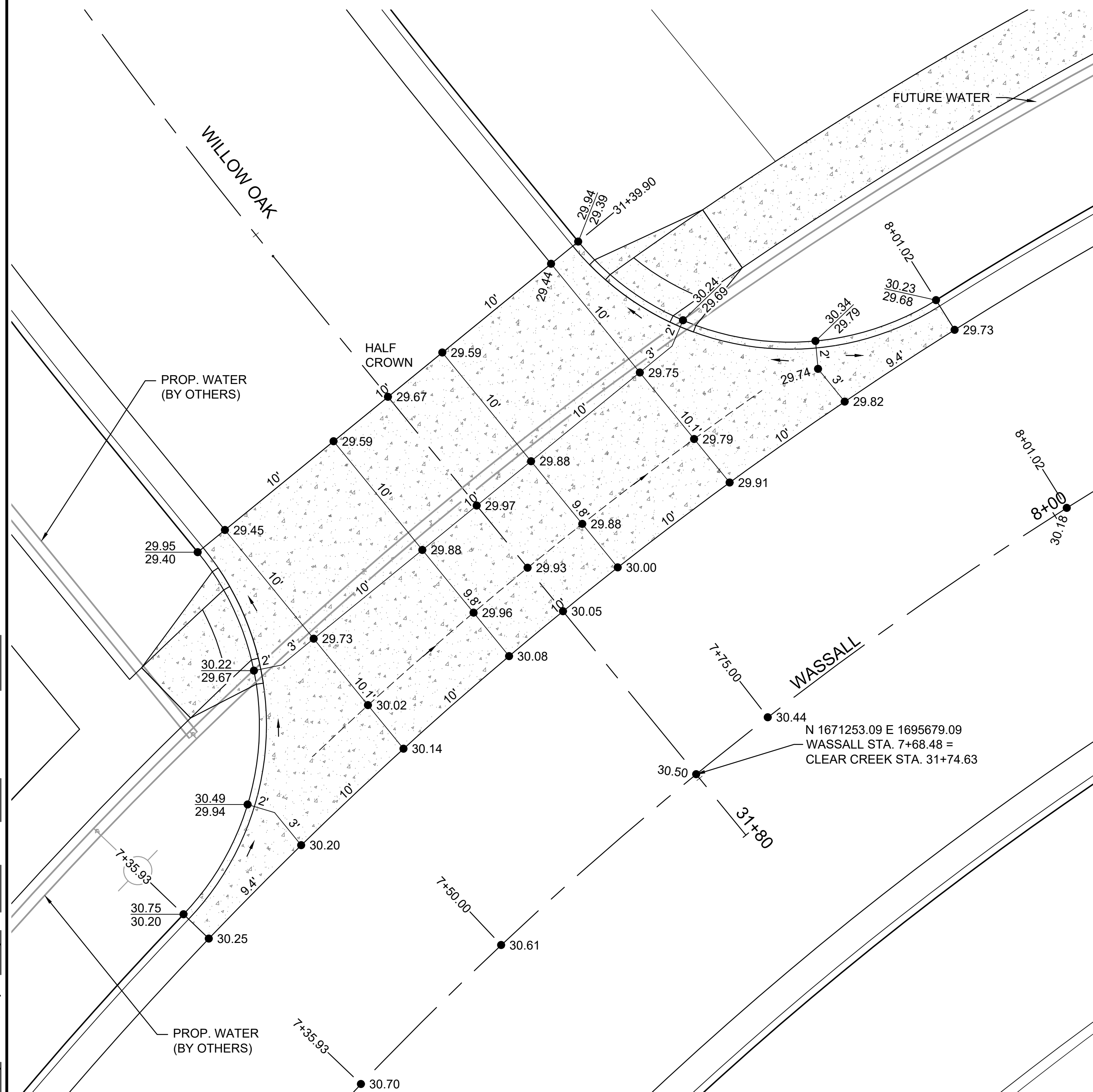
WILLOW OAK & WASSALL - VALLEY GUTTER DETAIL
