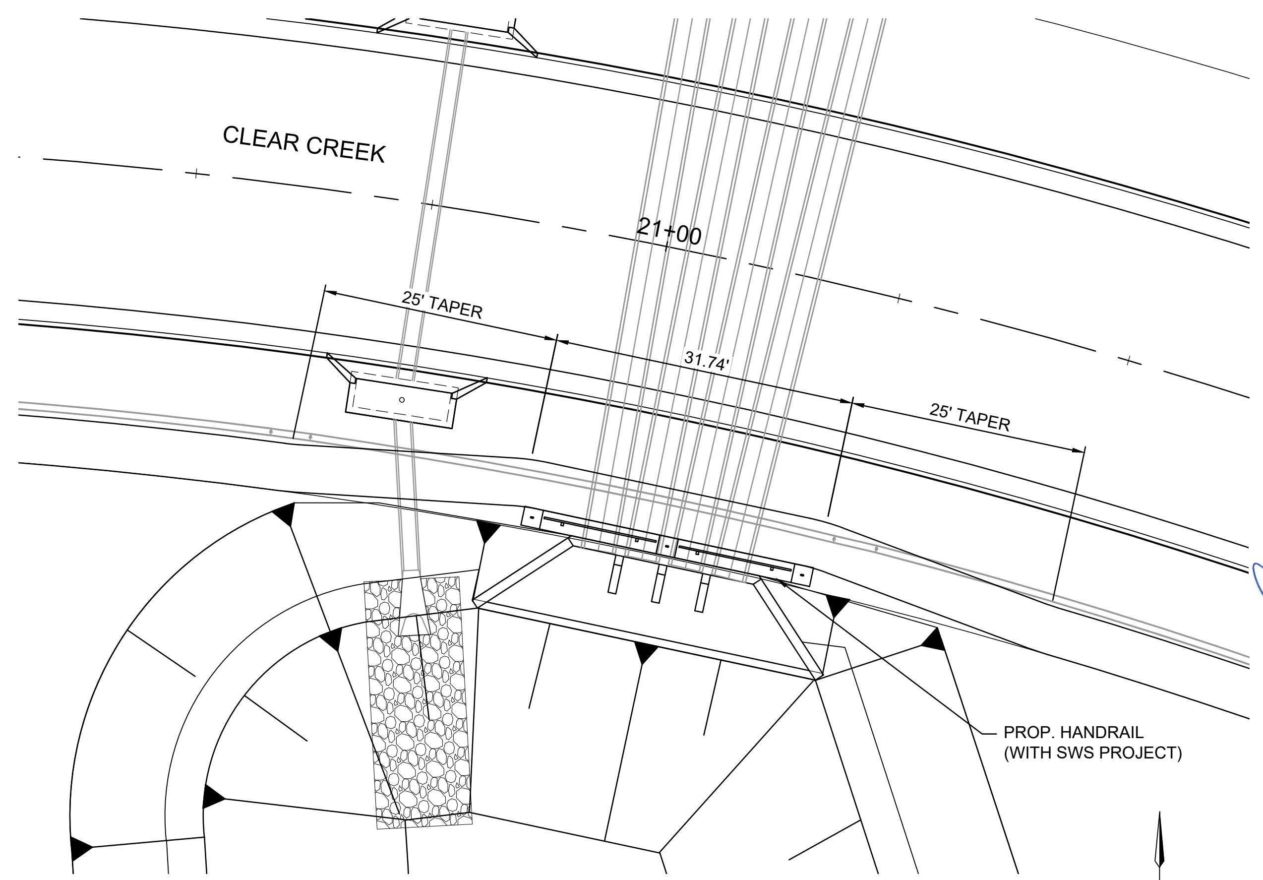
SIDEWALK DETAIL NEXT TO PEDESTRIAN RAIL
