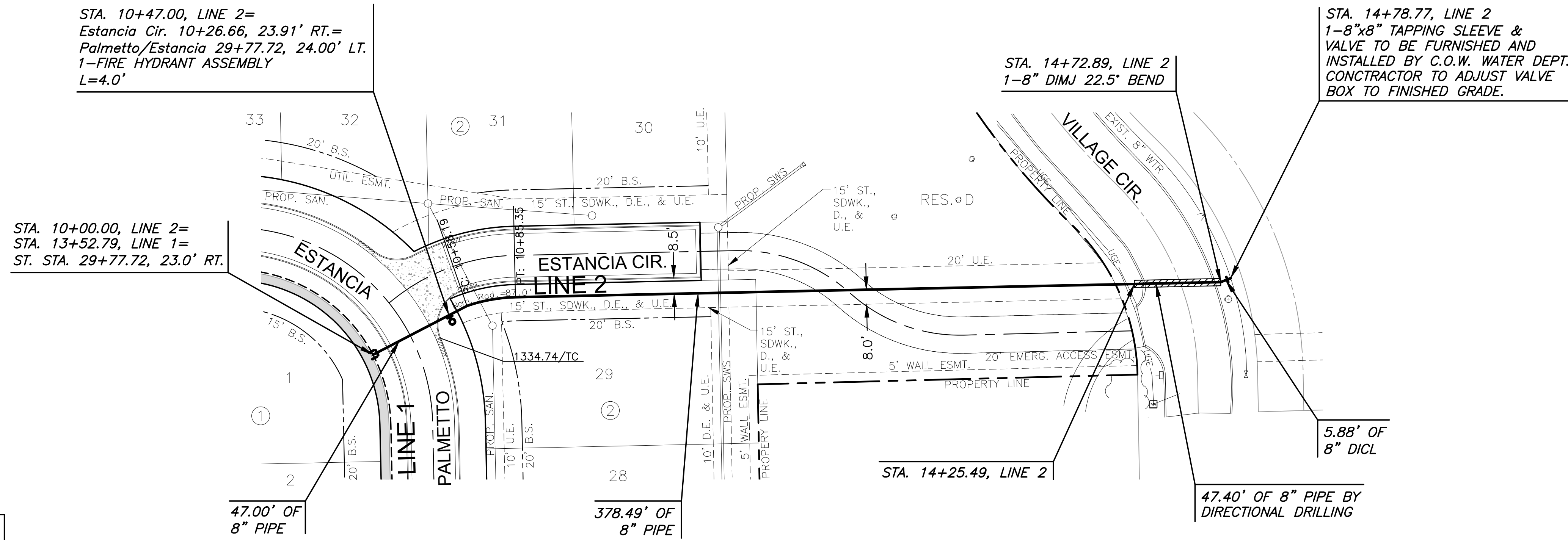
PLAN WTR LINE 2 PROFILE WTR LINE 2
