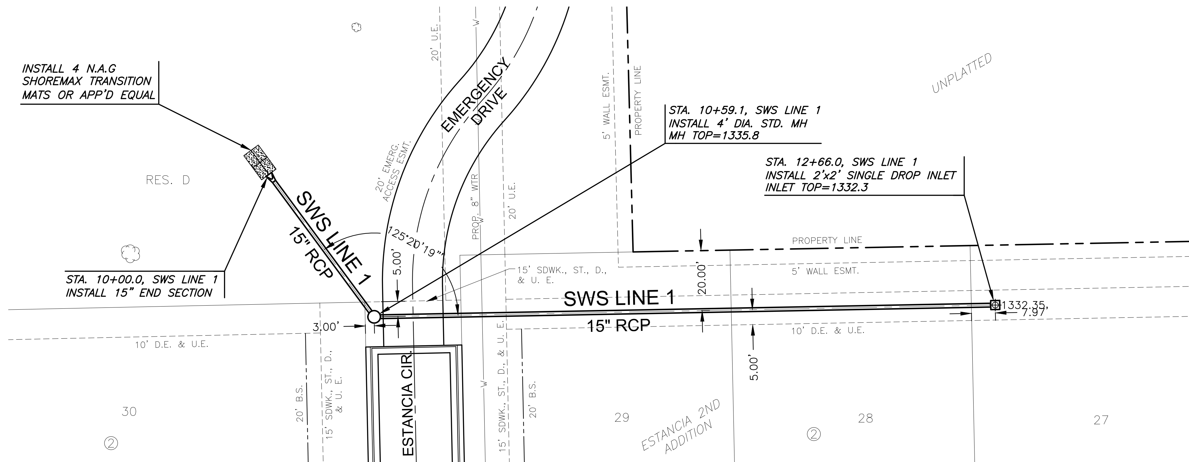
PLAN SWS LINE 1 PROFILE SWS LINE 1
