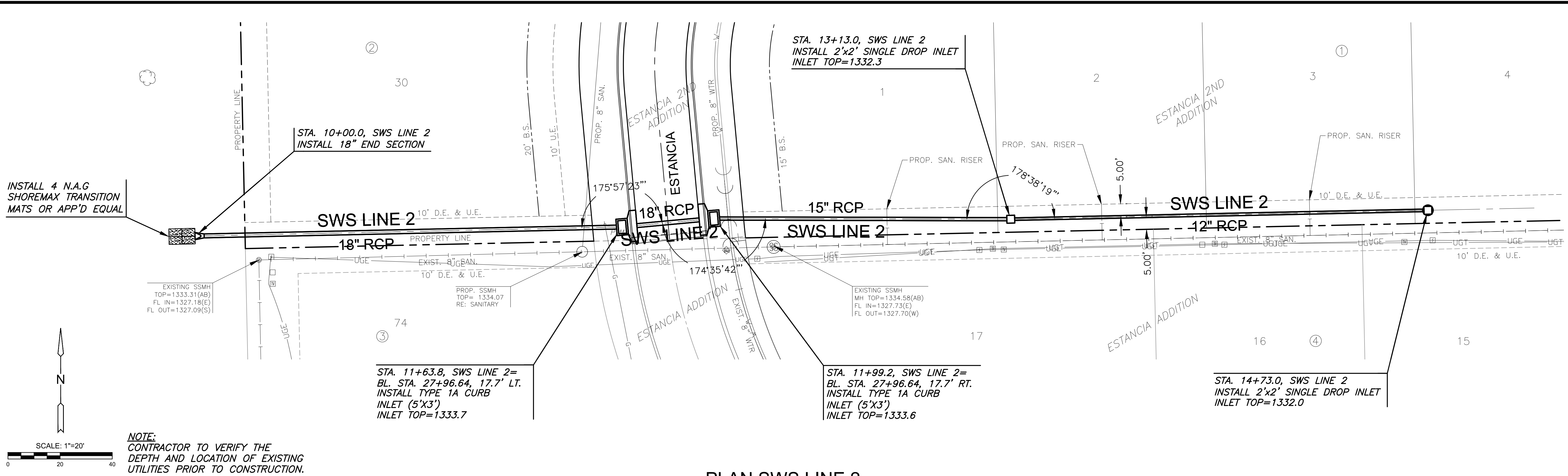
PLAN SWS LINE 2 PROFILE SWS LINE 2
