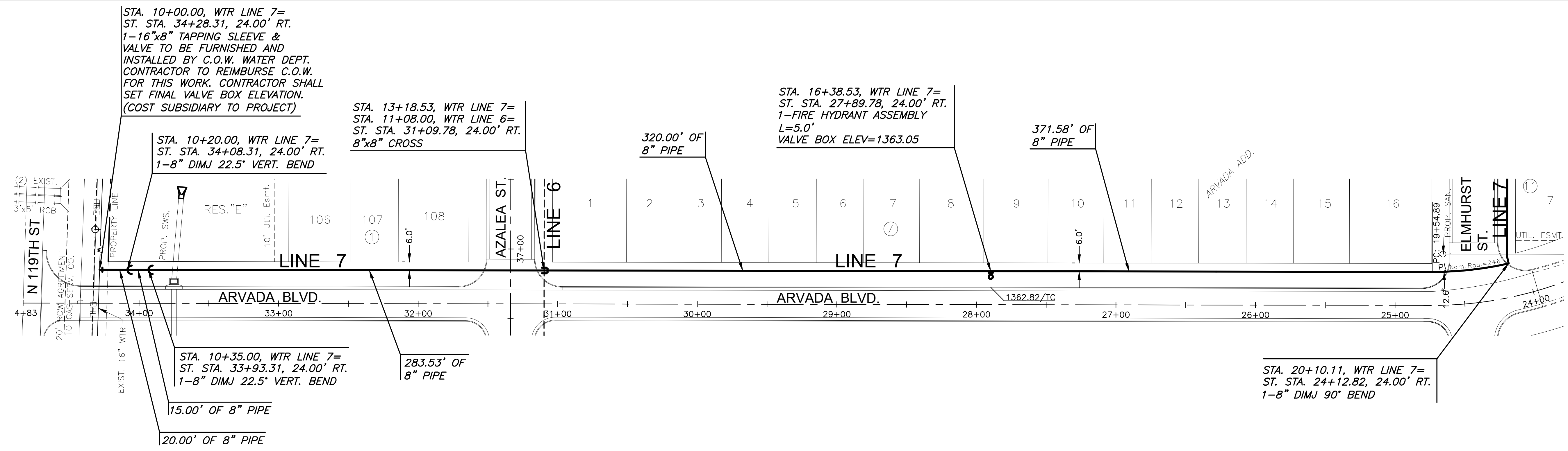
PLAN WTR LINE 7 PROFILE WTR LINE 7
