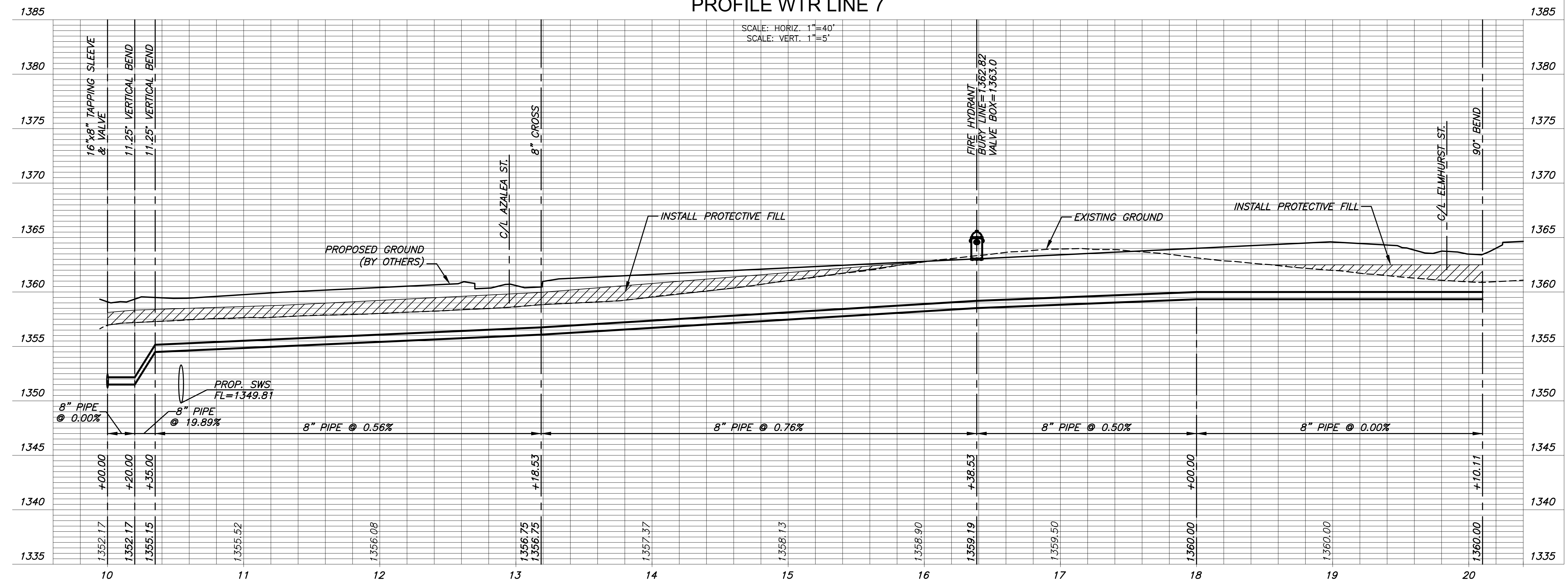
PLAN WTR LINE 7 PROFILE WTR LINE 7
