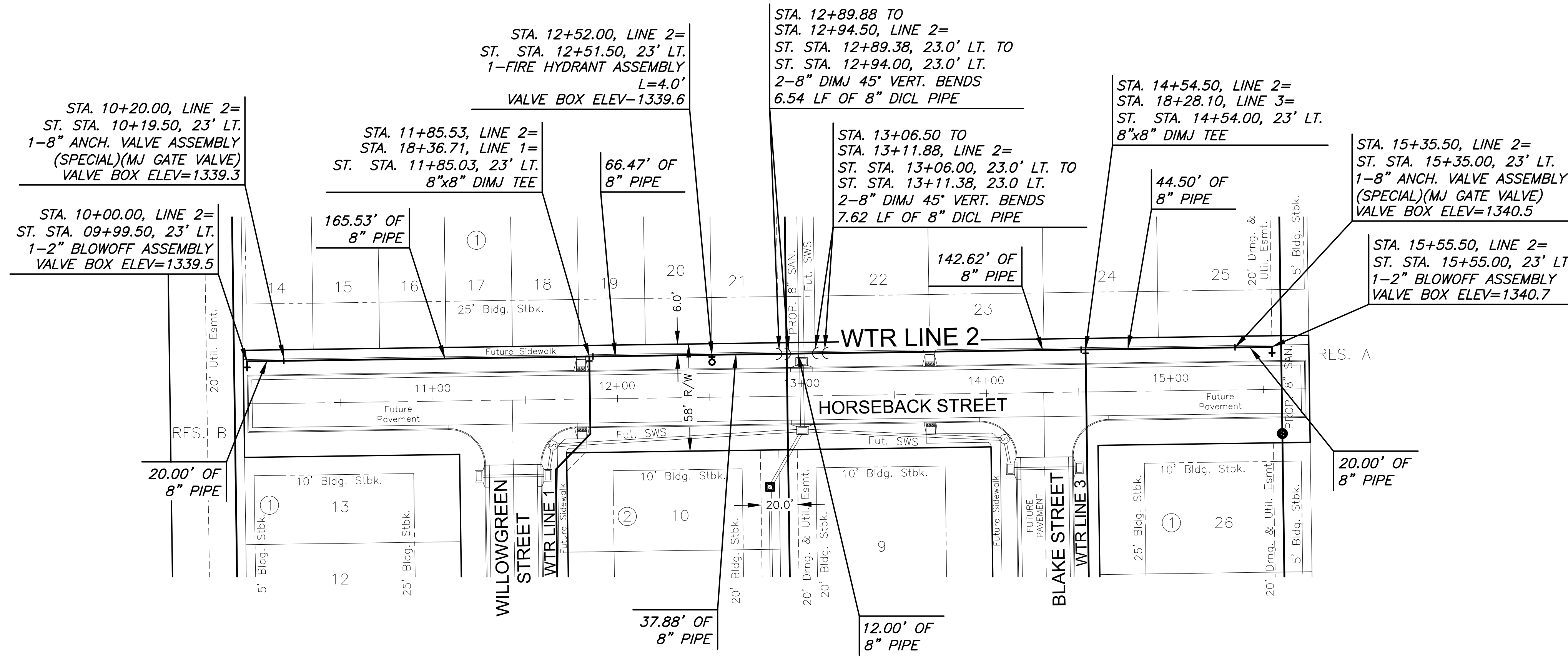
PLAN WTR LINE 2 PROFILE WTR LINE 2
