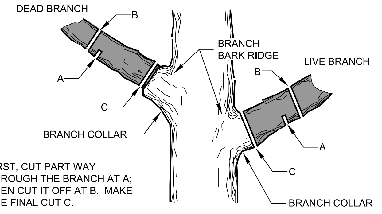
1 TREE TRIMMING DETAIL SCALE: NTS
