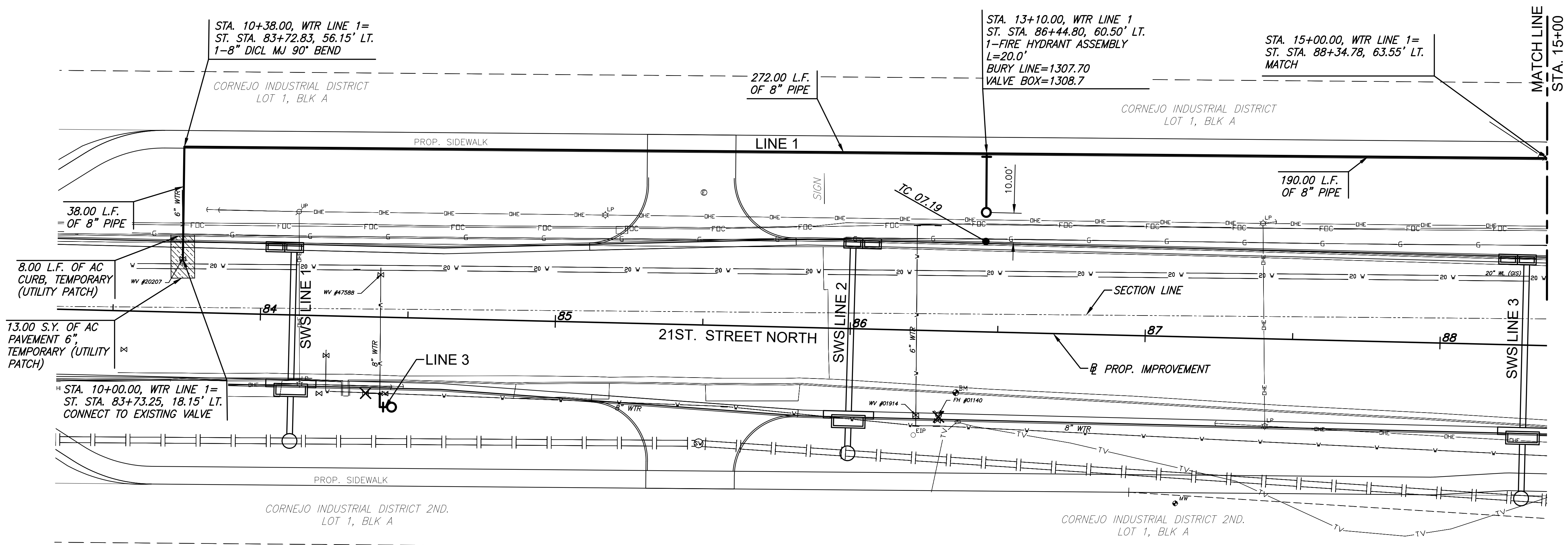
PLAN LINE 1 PH. 1 PROFILE LINE 1 PH. 1
