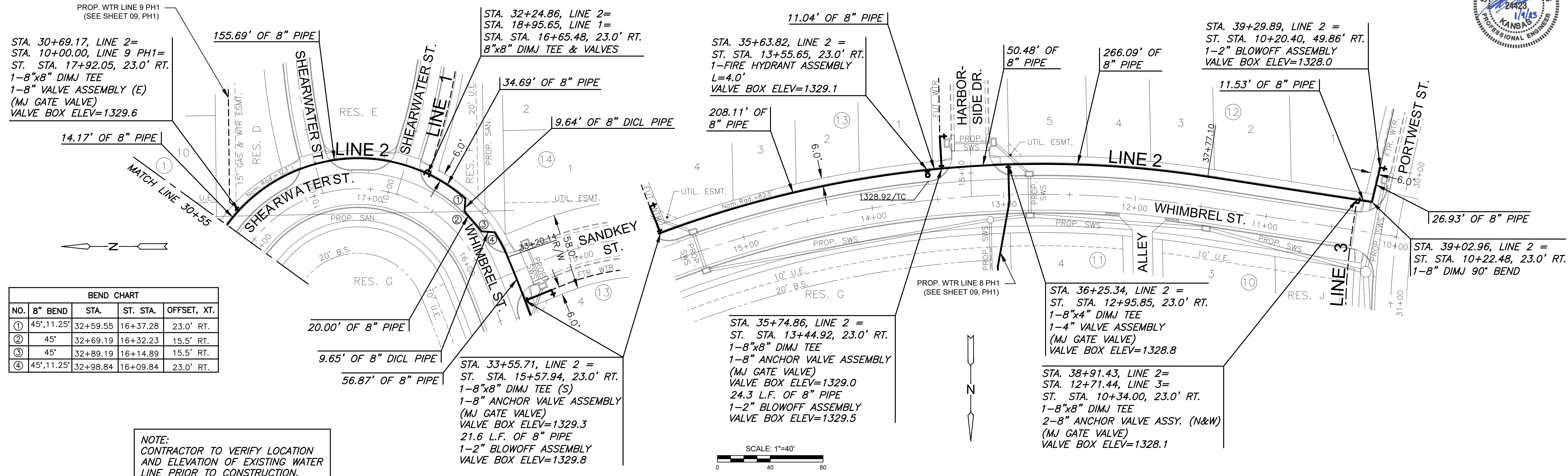
PLAN WTR LINE 2 COLLECTOR (CONT.) PROFILE WTR LINE 2 COLLECTOR (CONT.)
