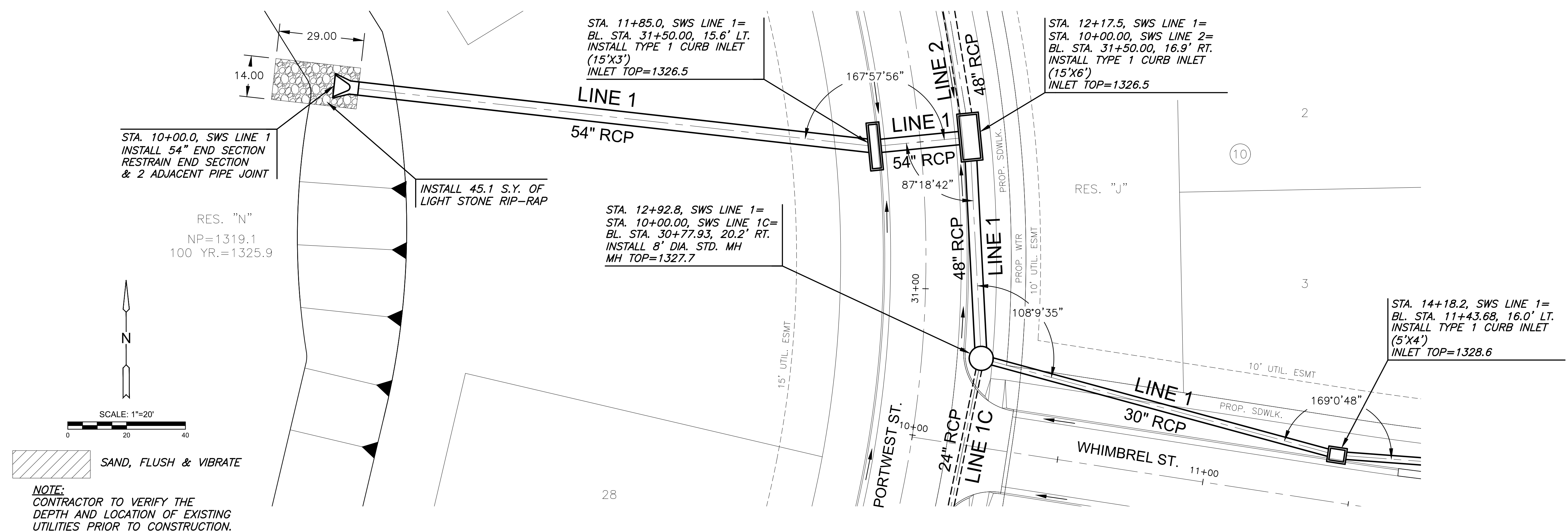
PLAN SWS LINE 1 PROFILE SWS LINE 1
