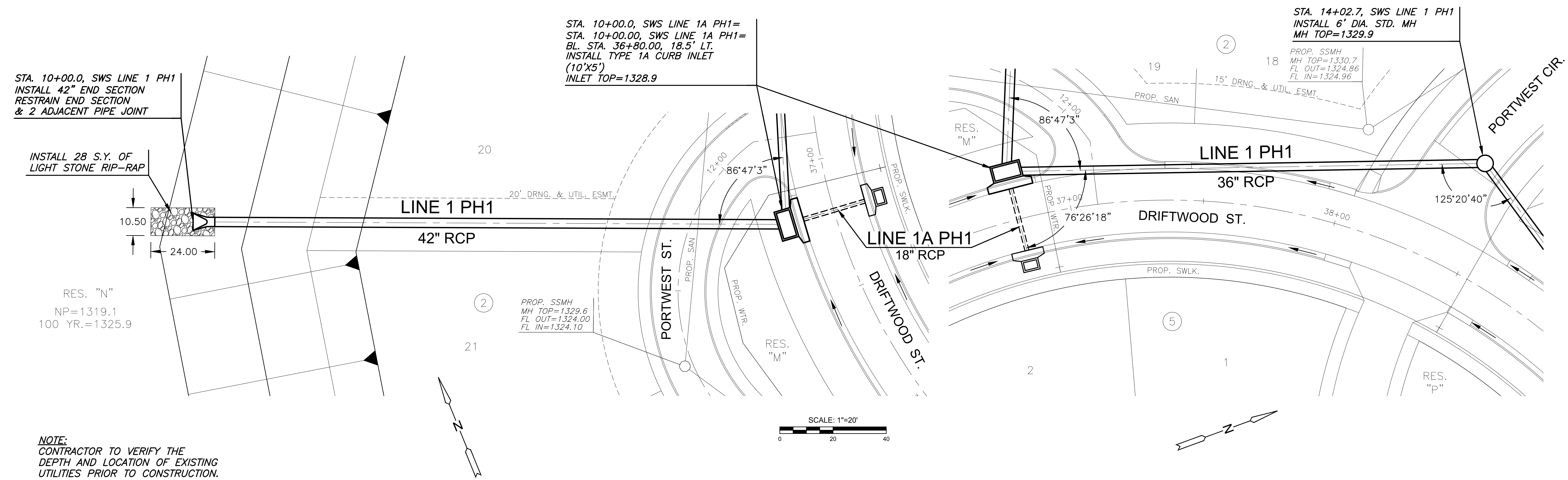
PLAN SWS LINE 1 PH1 PROFILE SWS LINE 1 PH1
