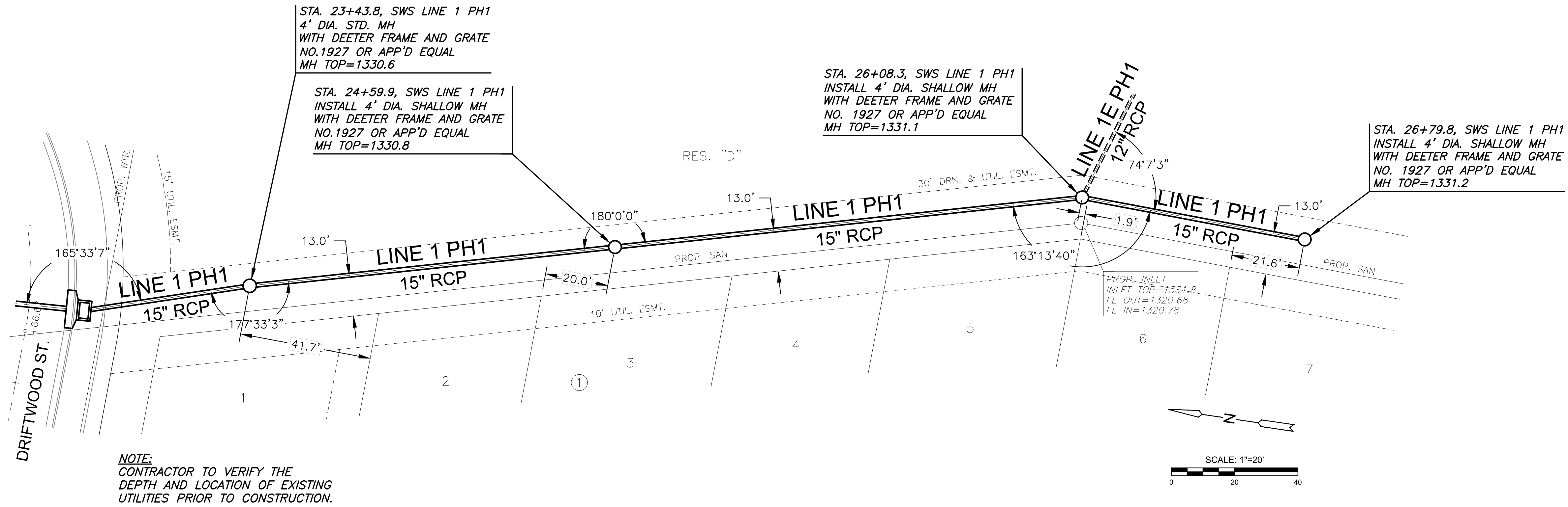
PLAN SWS LINE 1 PH1 (CONT. 3) PROFILE SWS LINE 1 PH1 (CONT. 3)
