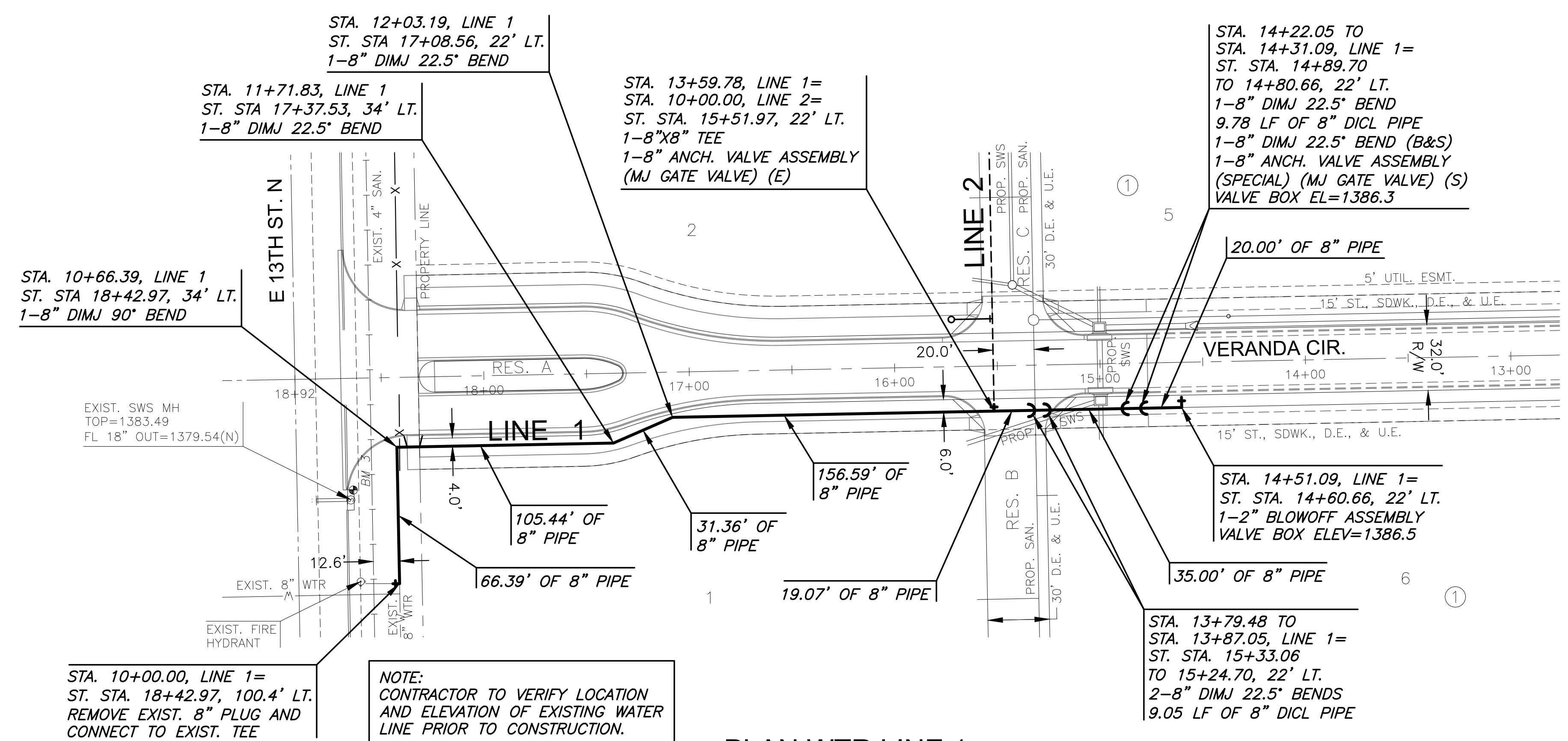
PLAN WTR LINE 1 PROFILE WTR LINE 1
