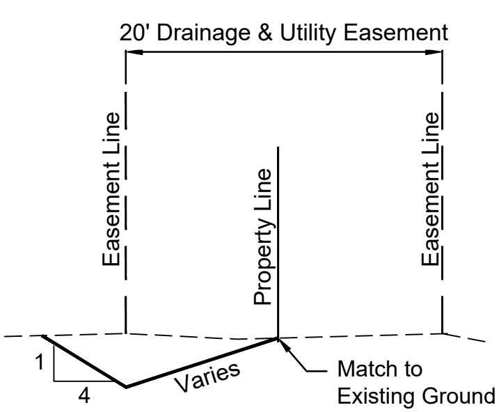
EASEMENT GRADING C-C
