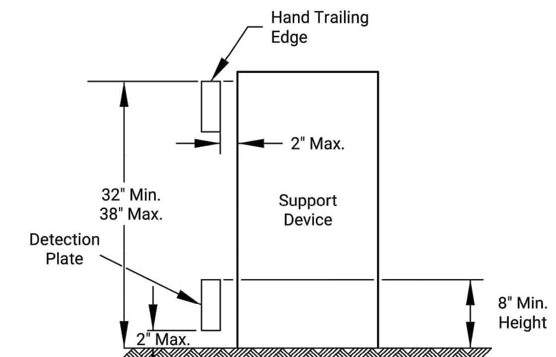
PEDESTRIAN CHANNELIZER Support device shall not project beyond the detection plate into the pathway. Hand trailing edges and detection plates are optional for continuous walls. Interconnect pedestrian channelizers to prevent displacement and to provide continuous guidance through or around work. Alternate pathways shall be firm, stable, and slip resistant. Treat height differentials > 1/2" in the surfaces of alternate paths with a firm, stable, and slip resistant temporary ramp having a slope of 12:1 or flatter and having a width equal to the alternate path. Use alternating orange/white on interconnected devices.
