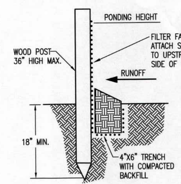
812 SILT FENCE BARRIERS
