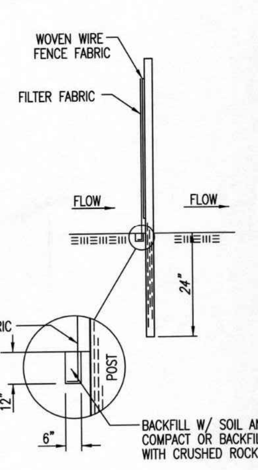
ANCHOR TRENCH DETAIL
