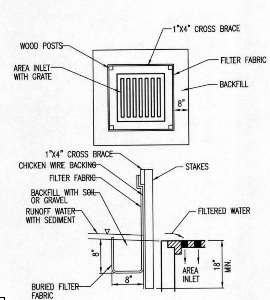
821 SILT FENCE BARRIERS FOR AREA INLETS (INLET PROTECTION)
