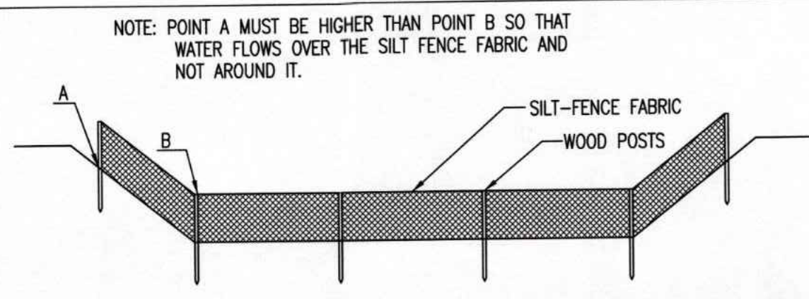
814 SILT FENCE DITCH CHECKS (STREAM PROTECTION)
