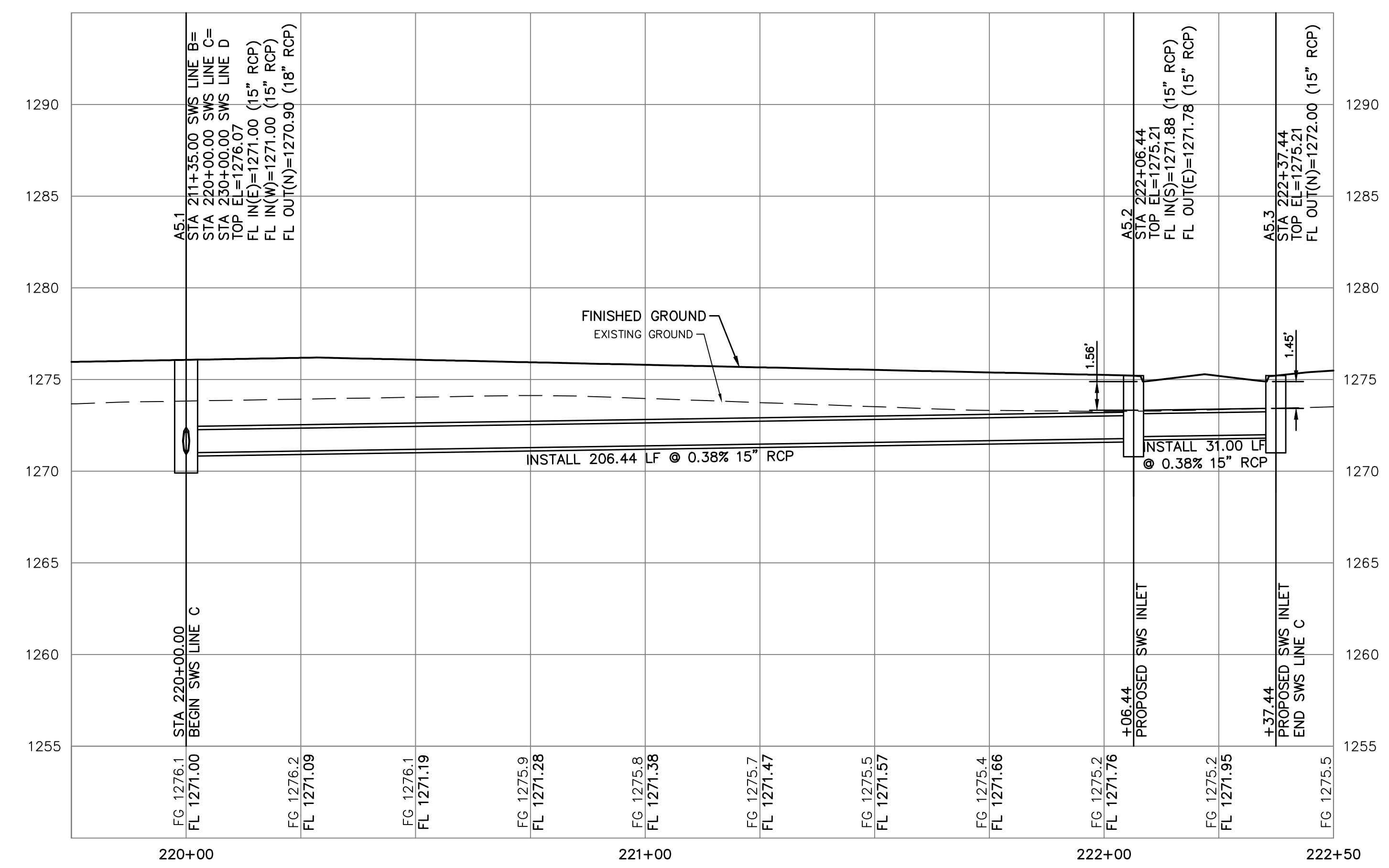
STORM WATER SEWER LINE C
