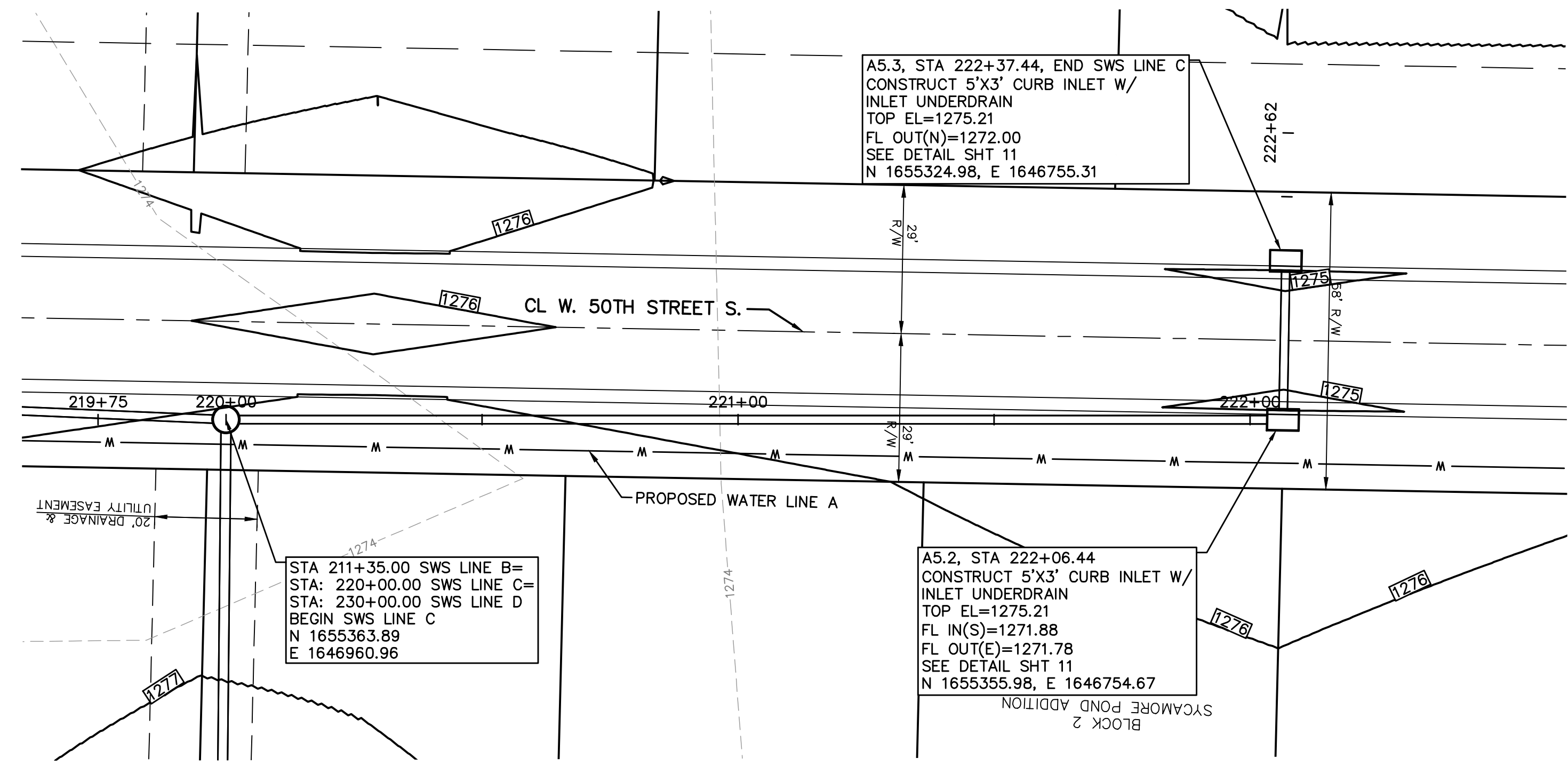
STORM WATER SEWER LINE C
