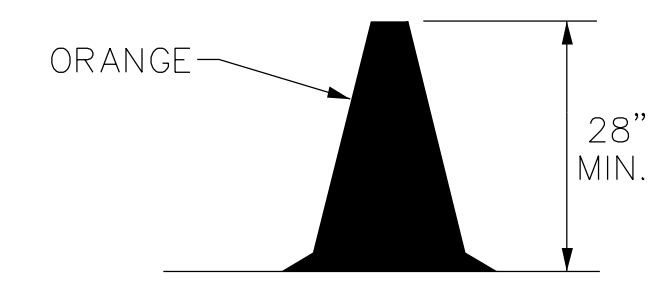
TRAFFIC CONE
