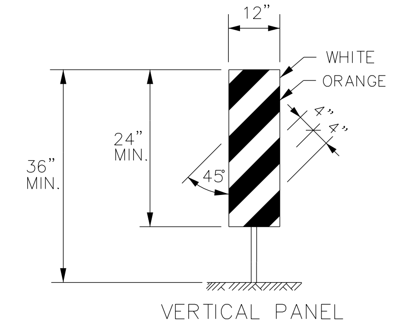
VERTICAL PANEL
