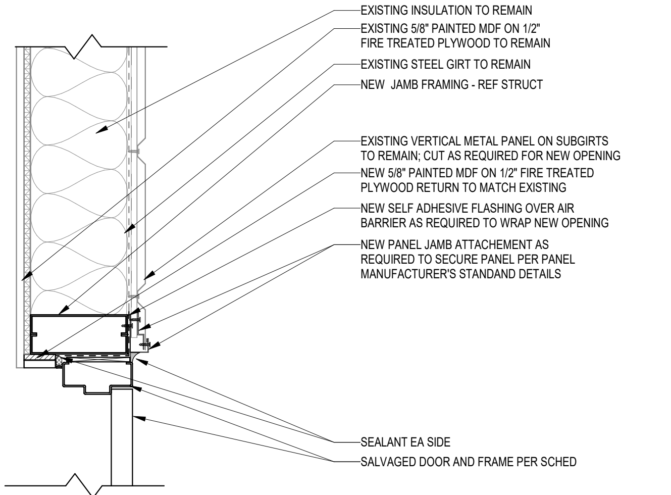
11 HM DOOR JAMB @ EXISTING PANEL 1 1/2" = 1'-0"
