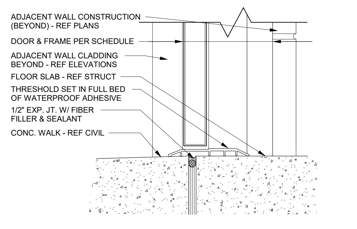
14 TYP THRESHOLD DETAIL 3" = 1'-0"
