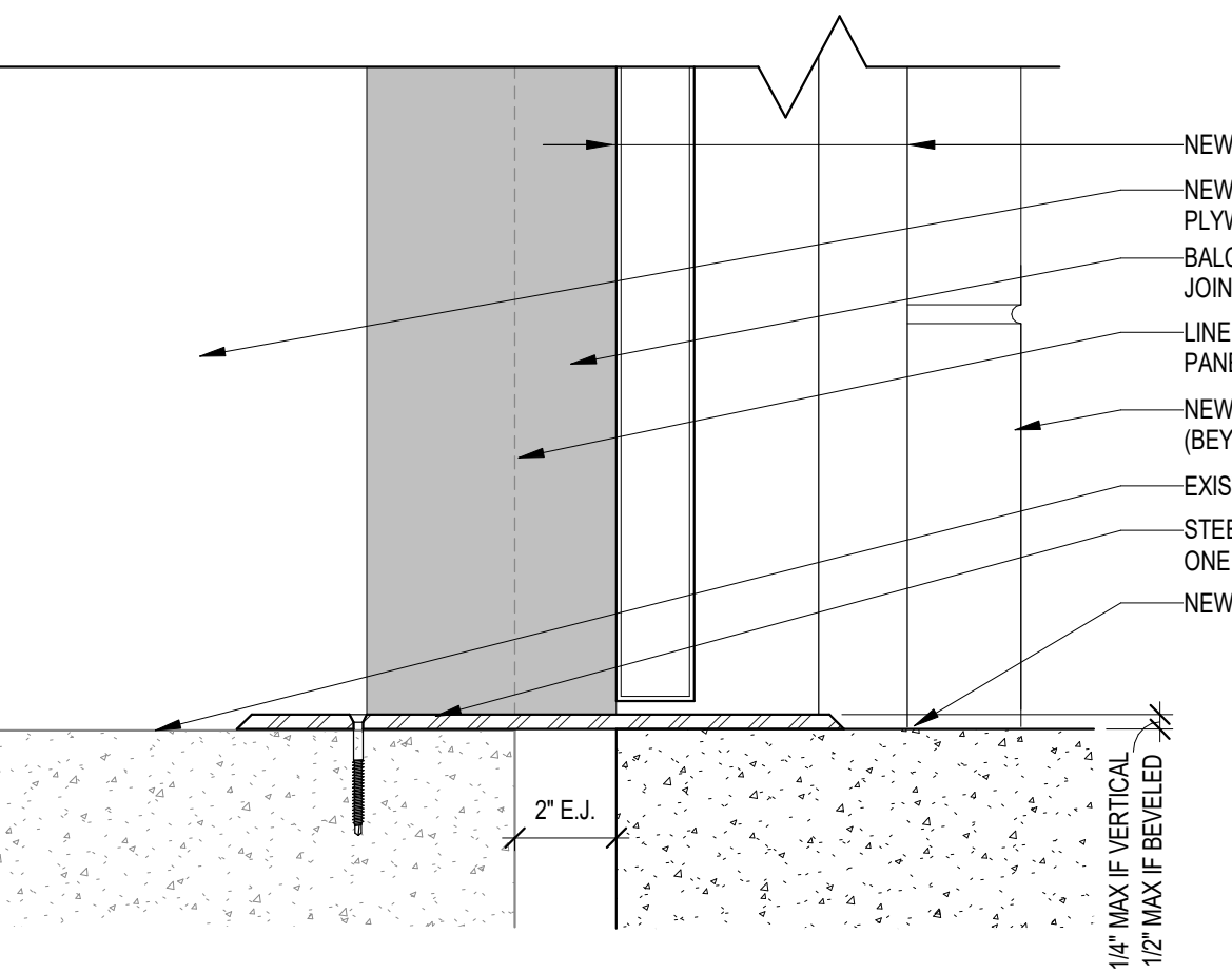
15 DOOR SILL @ EJ 3" = 1'-0"
