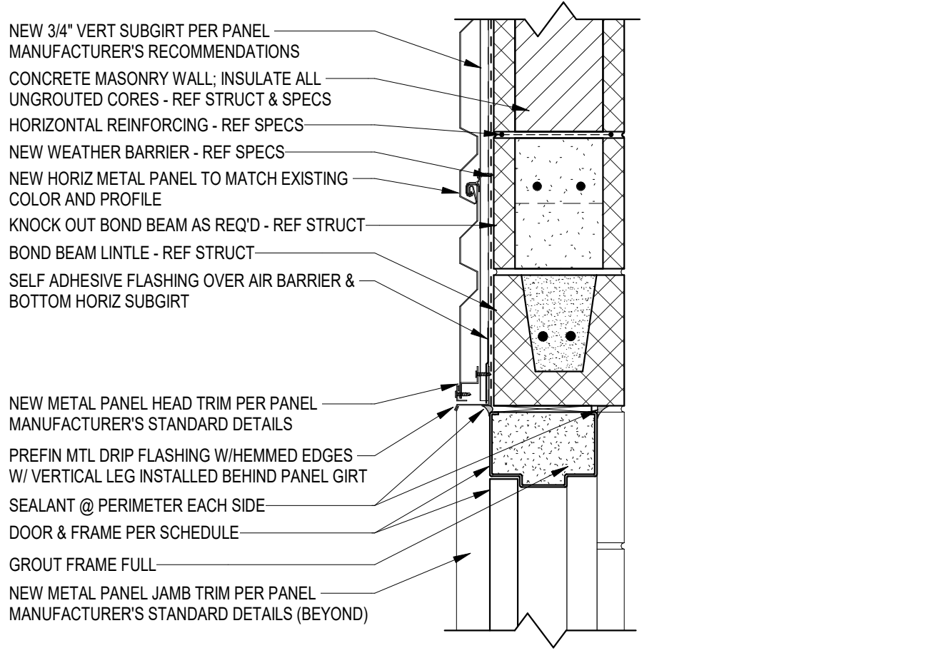
12 DOOR HEAD @ CMU & HORIZ MTL PANEL 1 1/2" = 1'-0"
