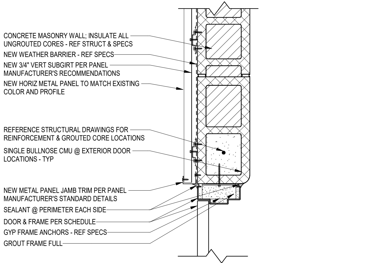
13 DOOR JAMB @ CMU & HORIZ MTL PANEL 1 1/2" = 1'-0"
