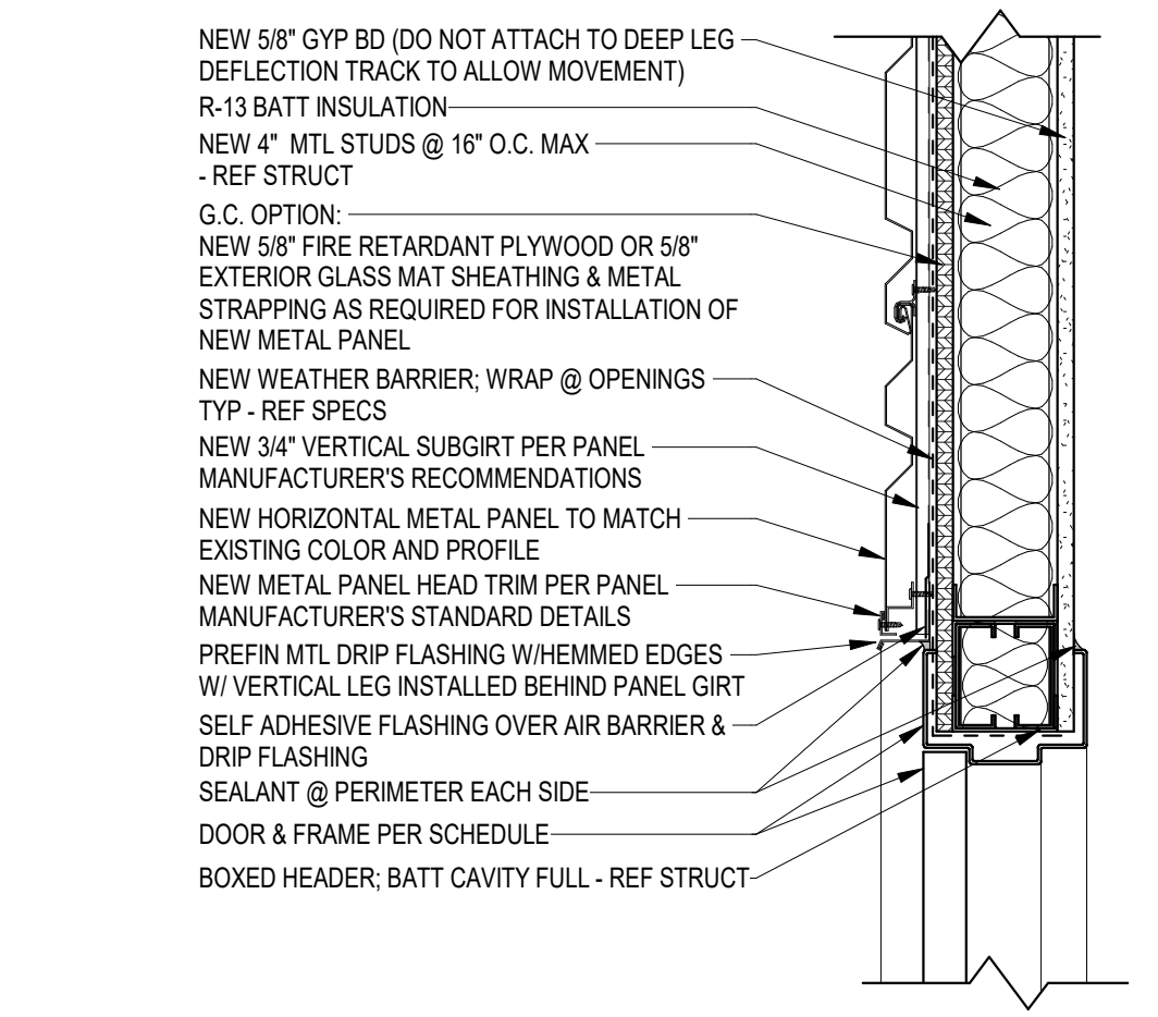
6 DOOR HEAD @ MTL PANEL 1 1/2" = 1'-0"
