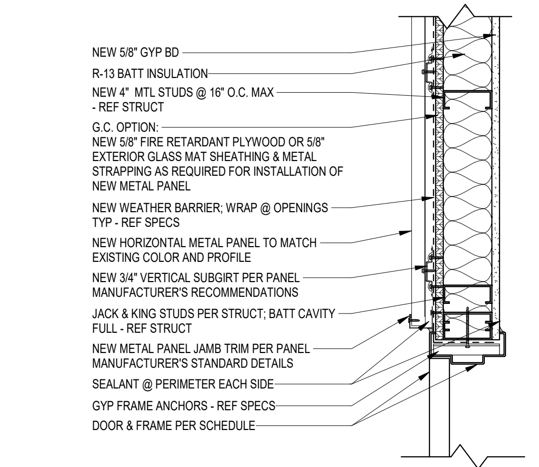
7 DOOR JAMB @ MTL PANEL 1 1/2" = 1'-0"
