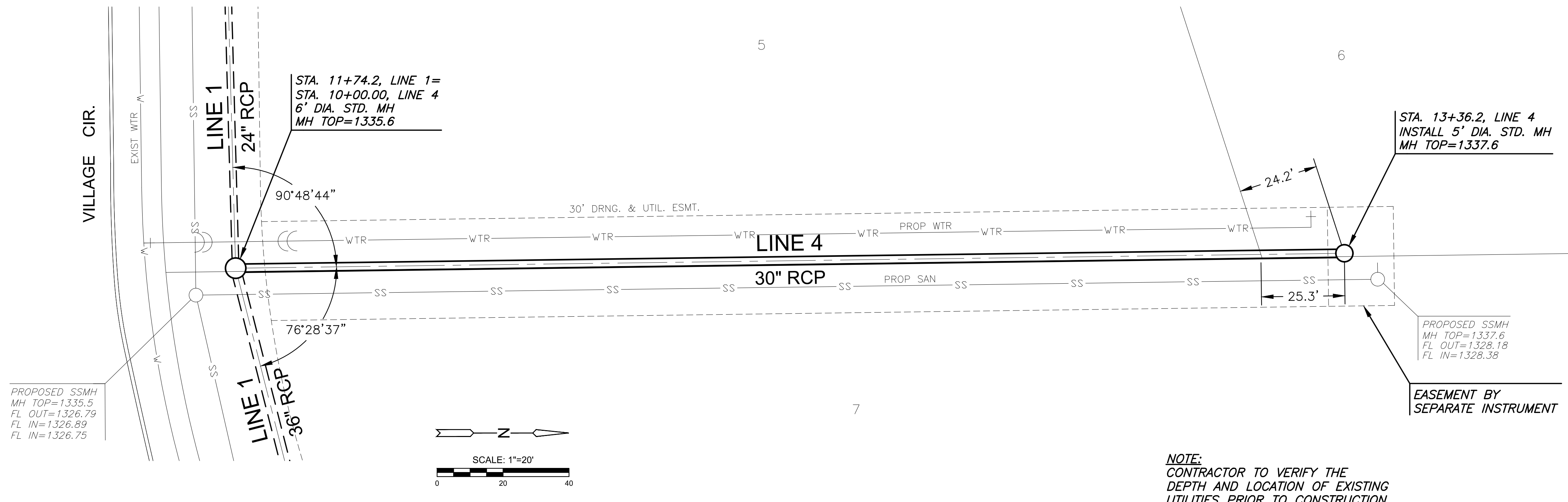
PLAN SWS LINE 4 PROFILE SWS LINE 4
