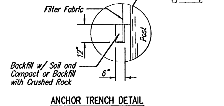
ANCHOR TRENCH DETAIL
