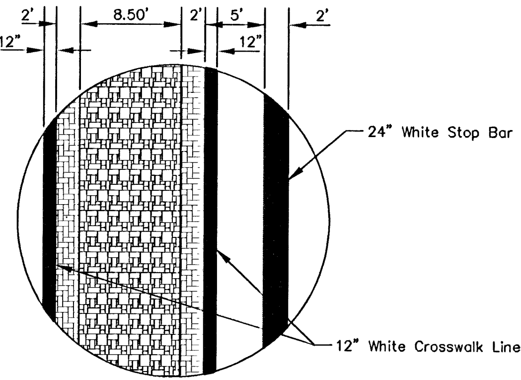
Crosswalk Detail
