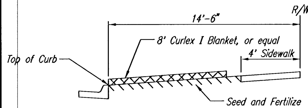
SECTION B-B
