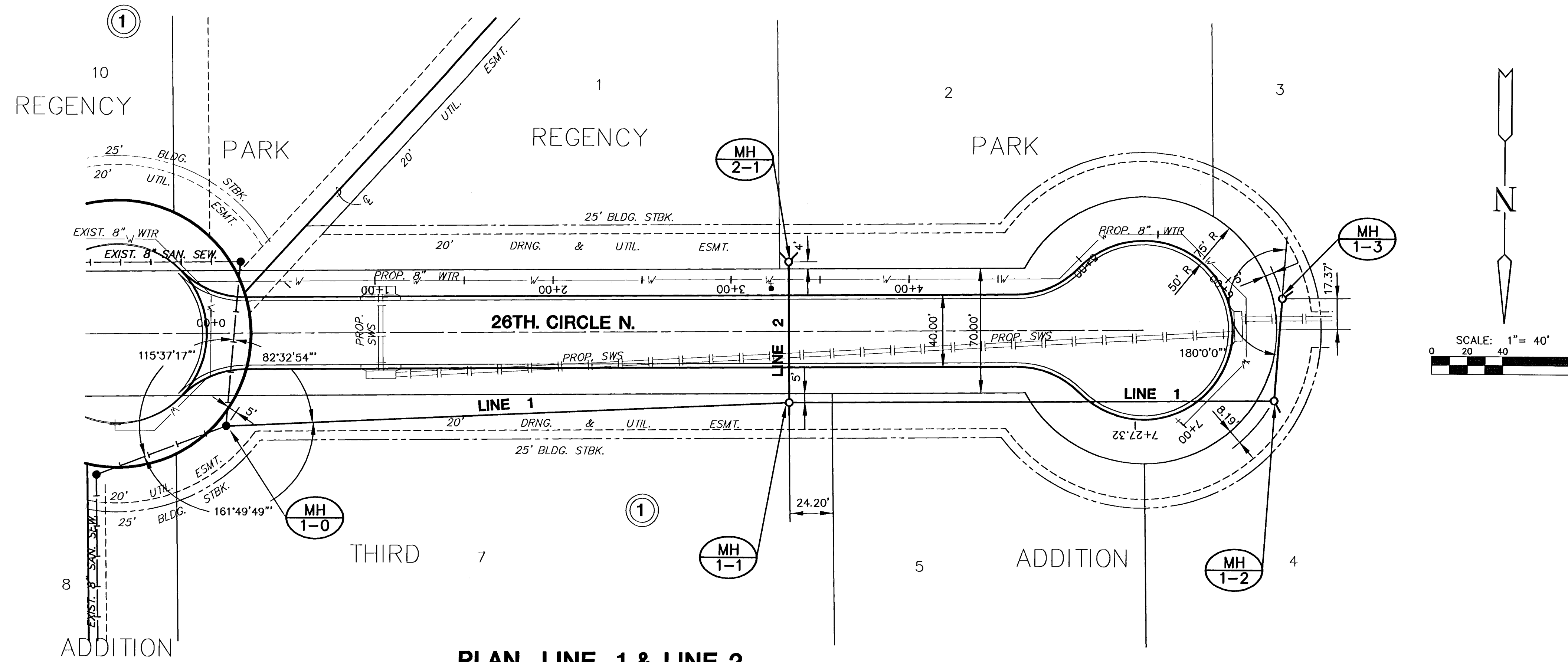
PLAN LINE 1 & LINE 2 SCALE: 1"=40'
